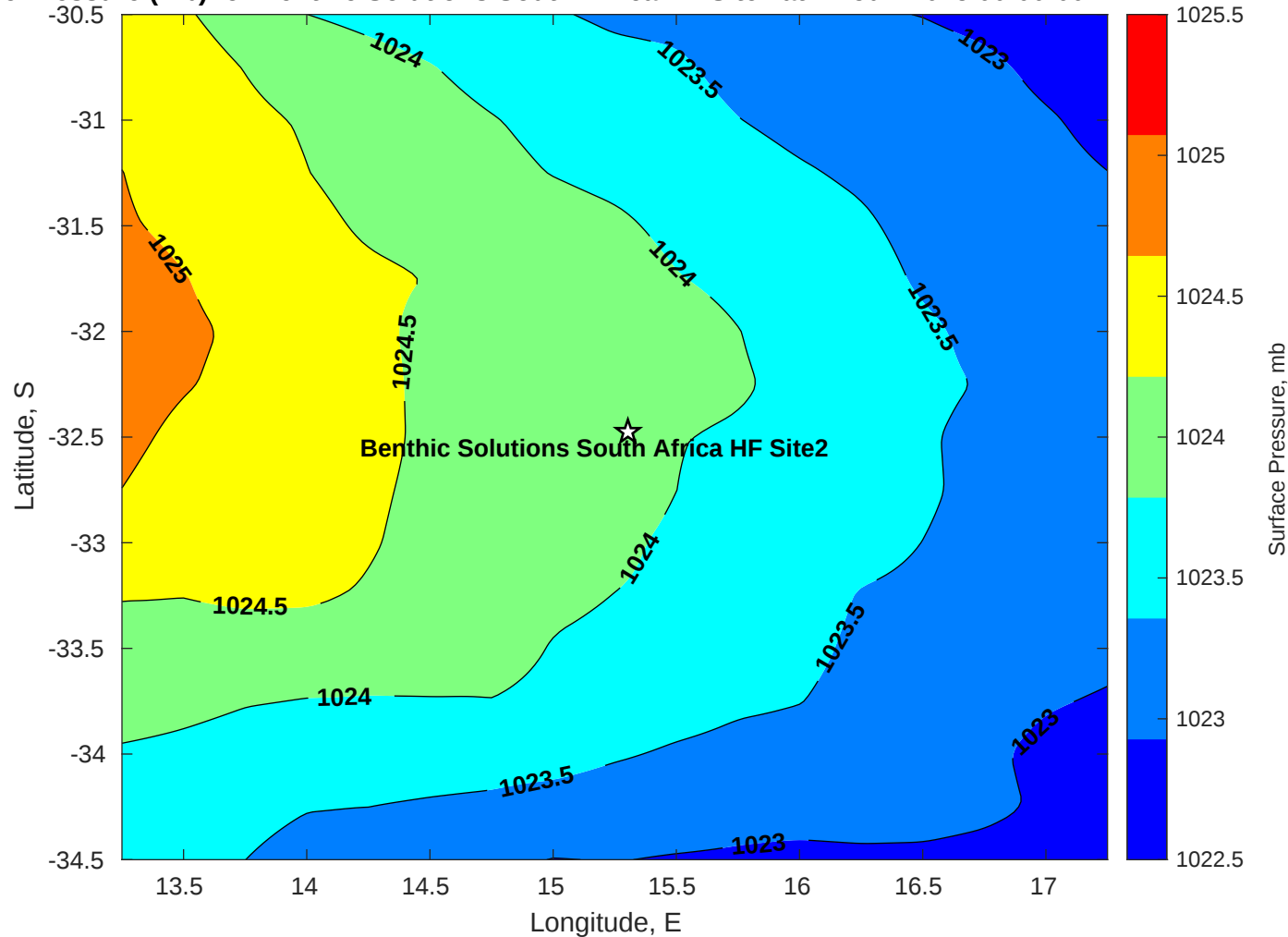
Surface Pressure (mb) for Benthic Solutions South Africa HF Site2 at 17-Jun-2025 00:00:00
