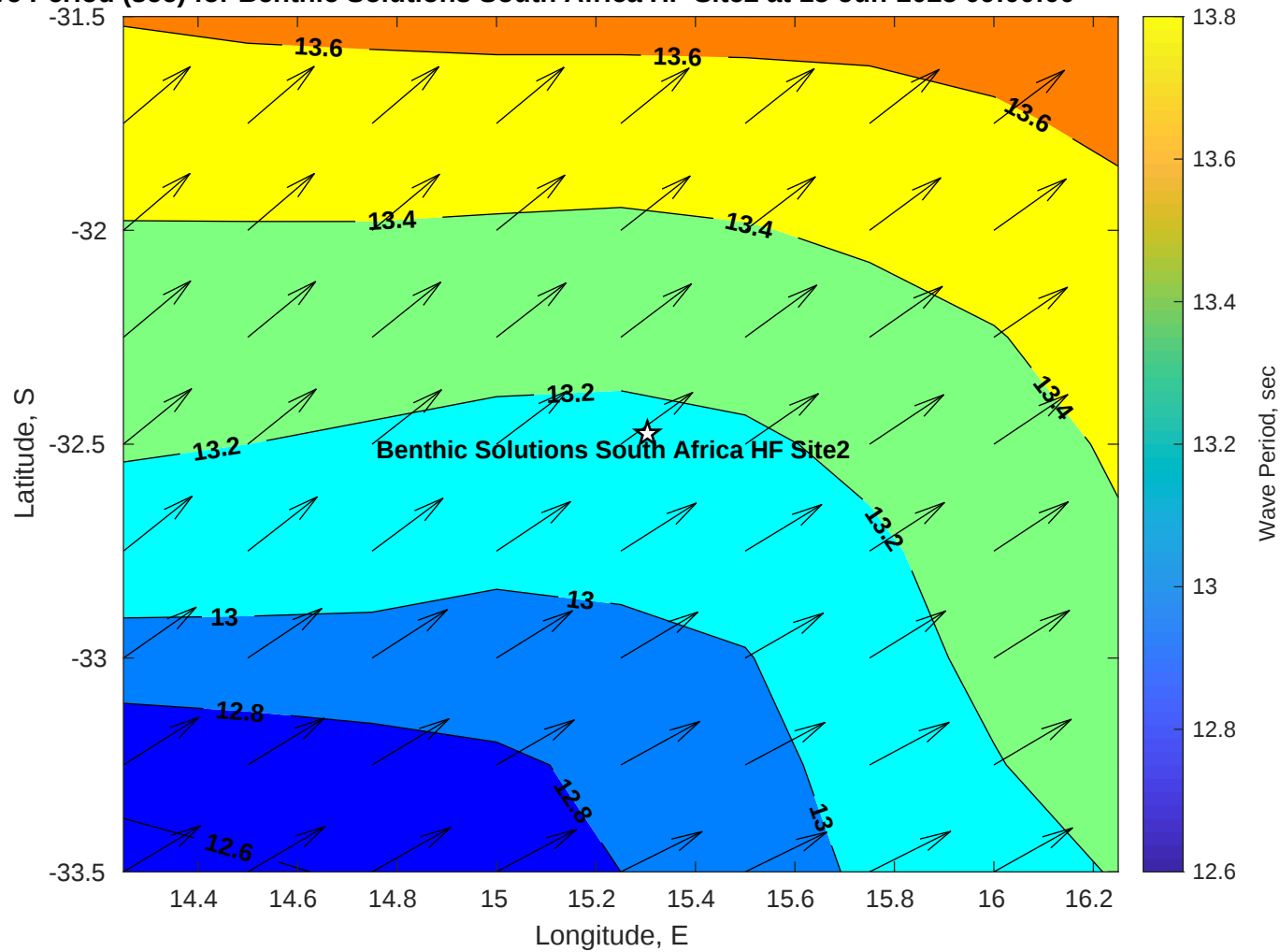
Wave Period (sec) for Benthic Solutions South Africa HF Site2 at 15-Jun-2025 09:00:00
