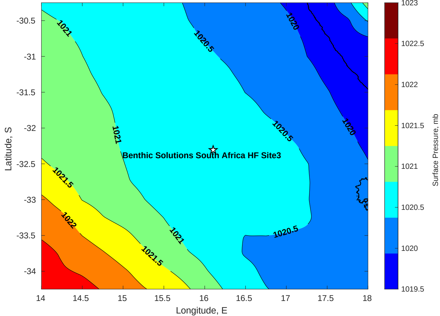
Surface Pressure (mb) for Benthic Solutions South Africa HF Site3 at 16-Jun-2025 00:00:00
