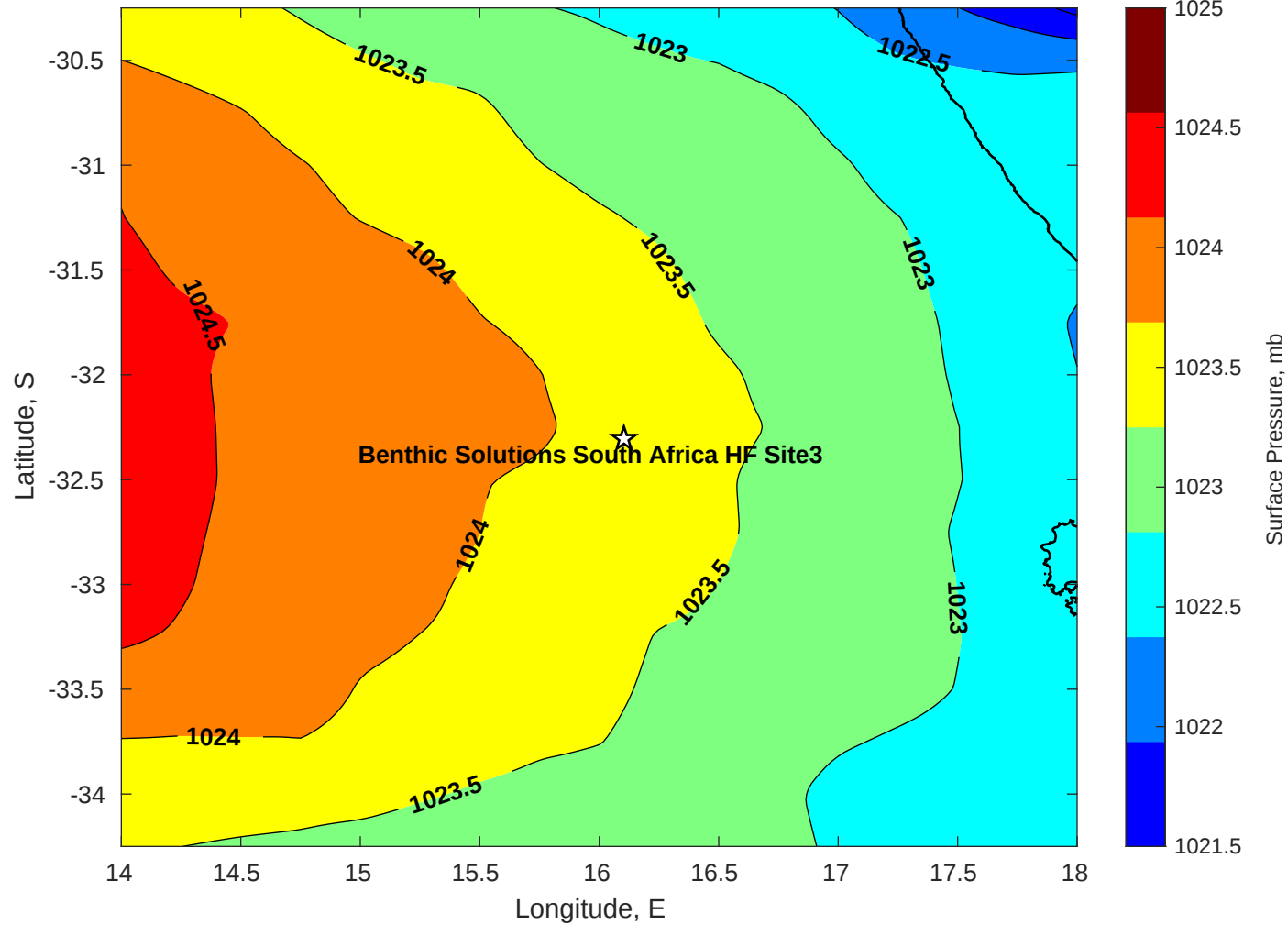
Surface Pressure (mb) for Benthic Solutions South Africa HF Site3 at 17-Jun-2025 00:00:00
