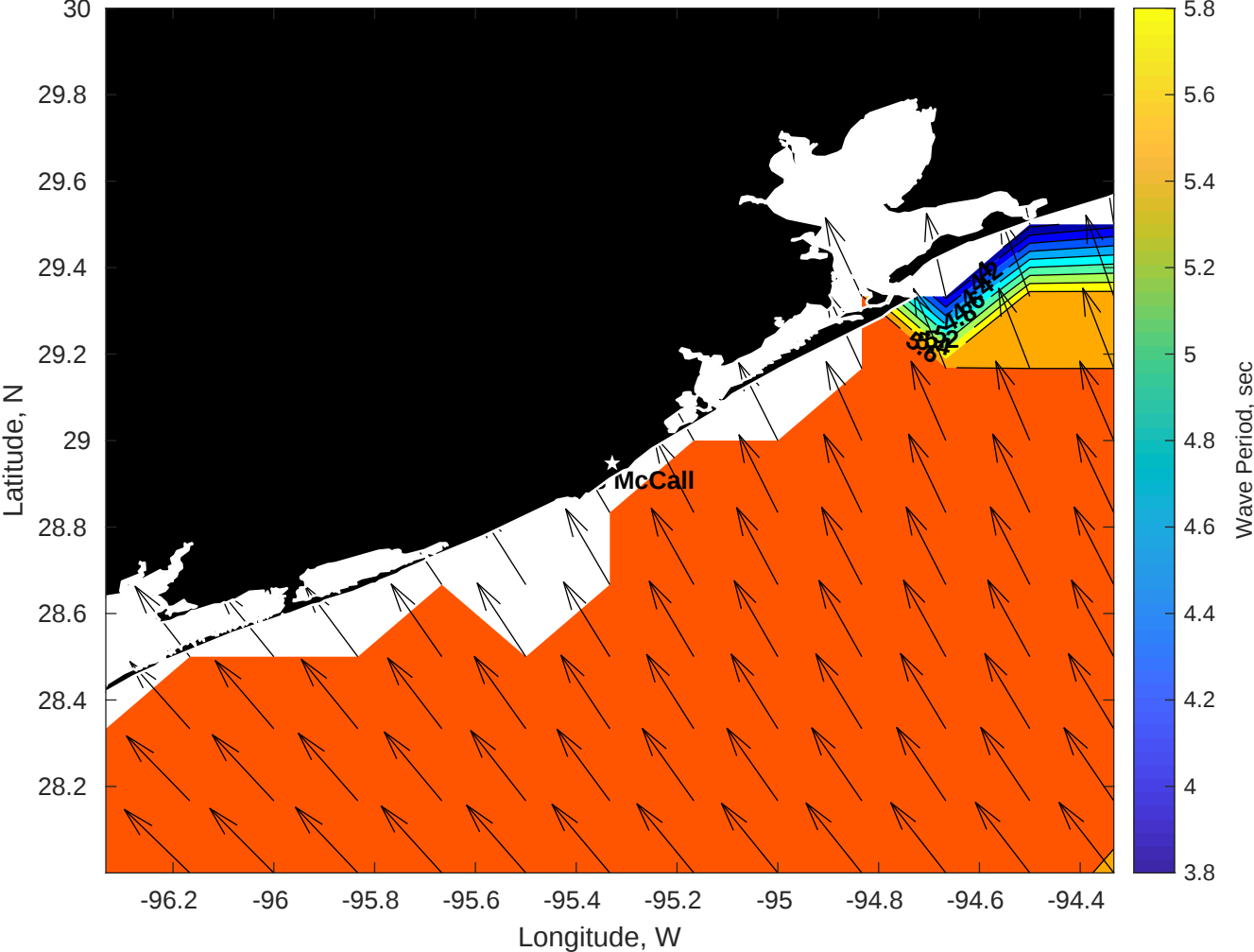
Wave Period (sec) for Brooks McCall at 16-Jun-2025 09:00:00
