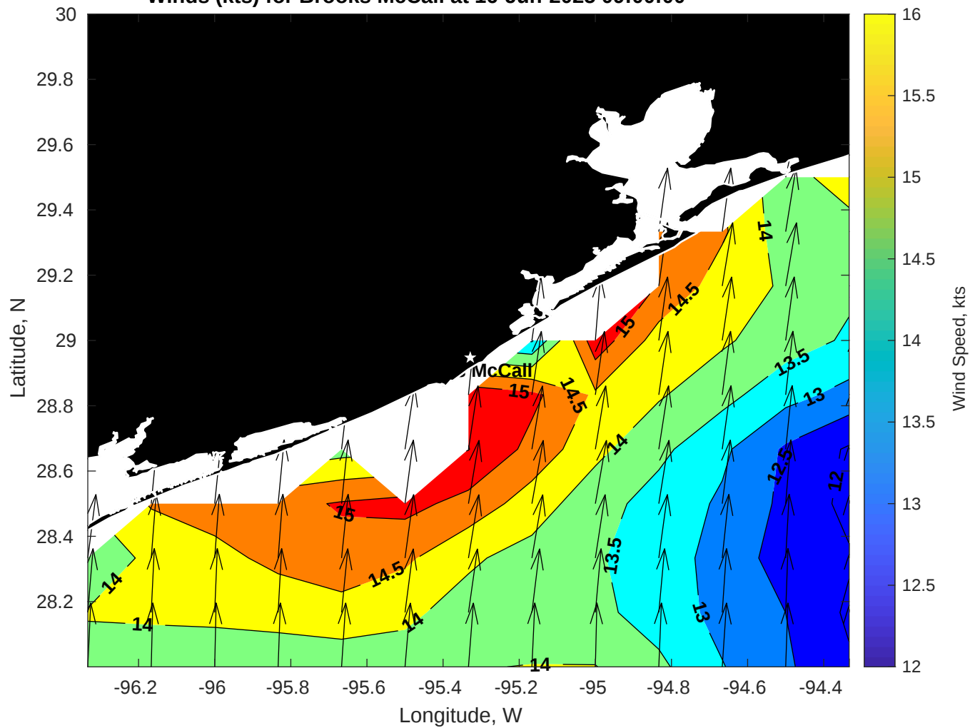
Winds (kts) for Brooks McCall at 16-Jun-2025 09:00:00
