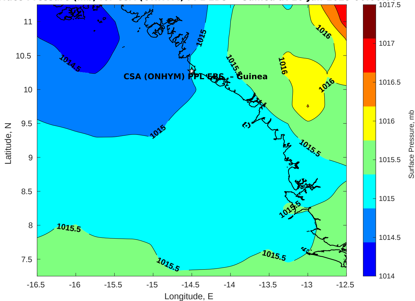
Surface Pressure (mb) for CSA (ONHYM) PPL EBS - Guinea at 16-Jun-2025 00:00:00
