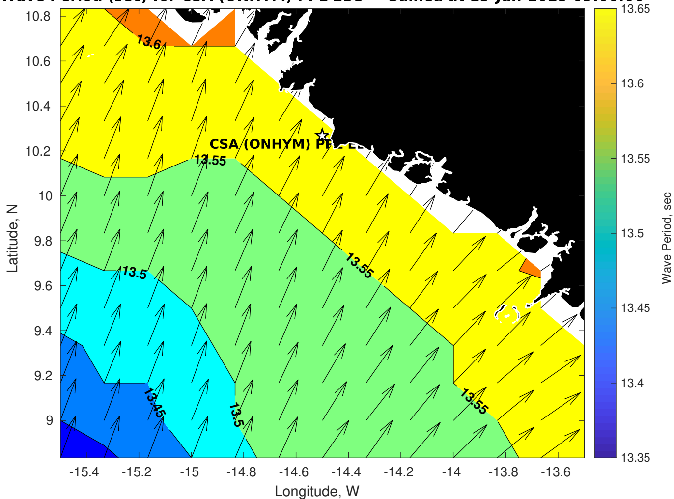
Wave Period (sec) for CSA (ONHYM) PPL EBS - Guinea at 15-Jun-2025 09:00:00
