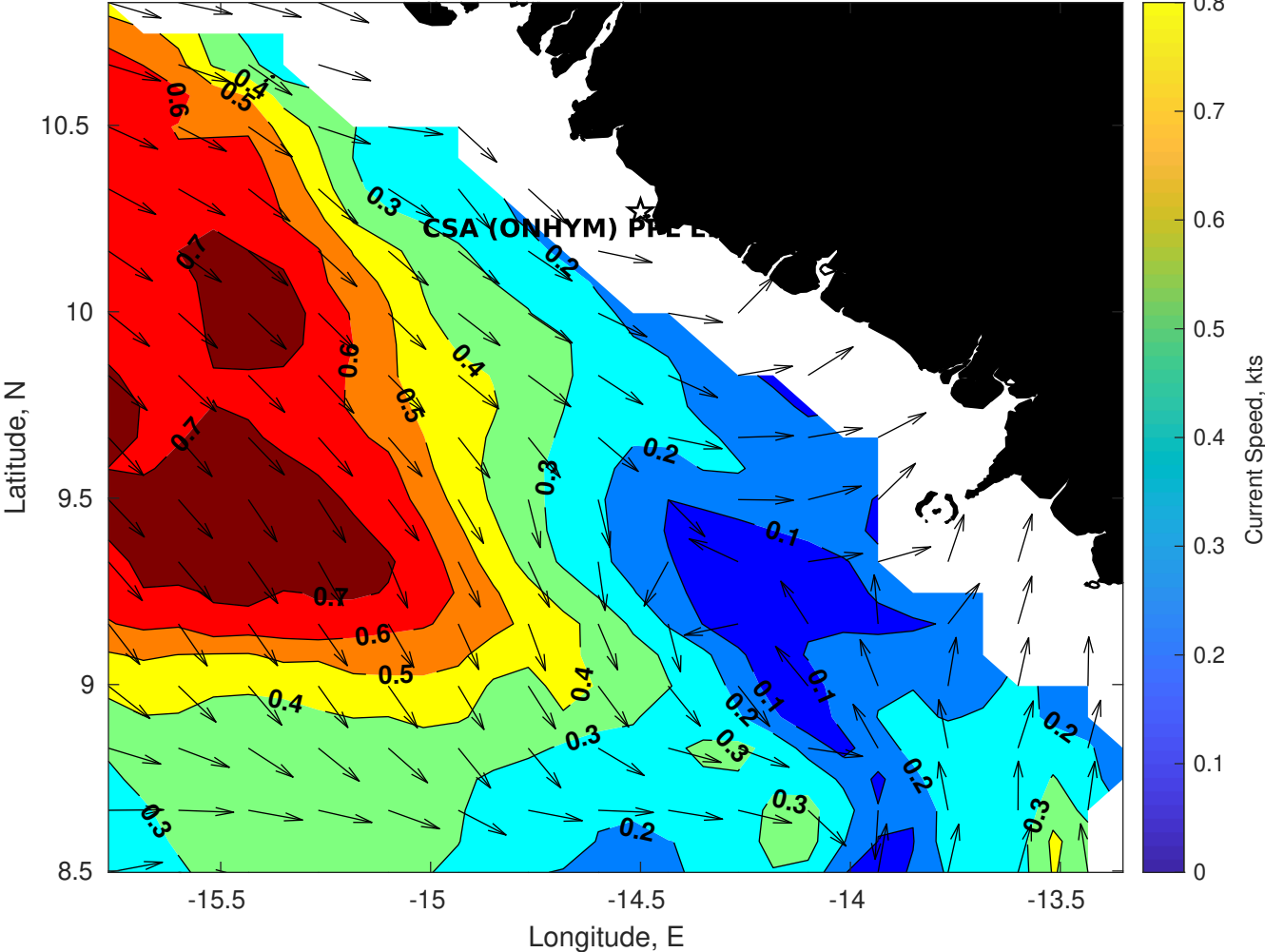
Surface Currents for CSA (ONHYM) PPL EBS - Guinea at 07-Jun-2025 00:00:00
