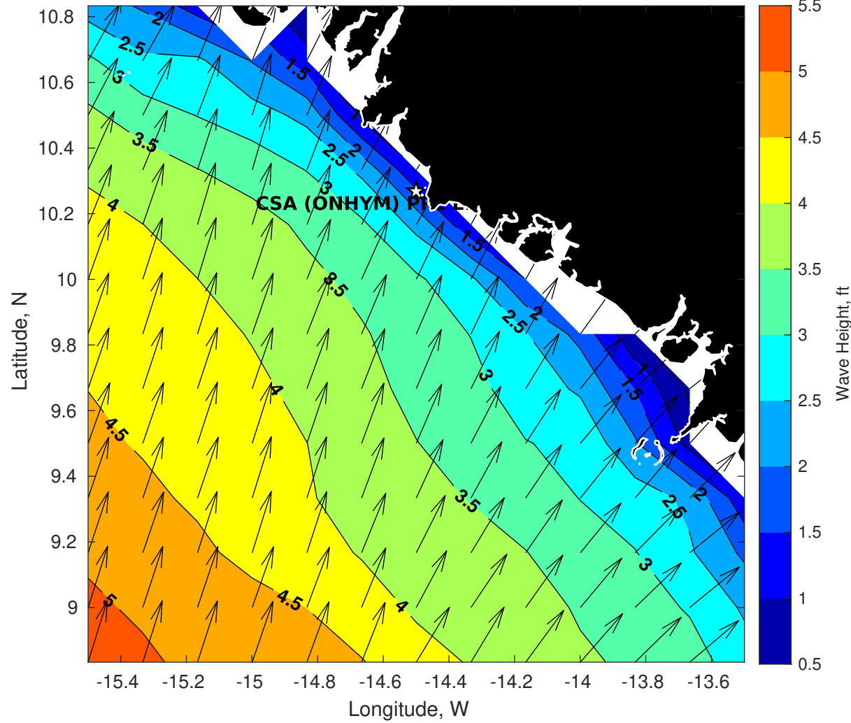
Wave Height (ft) for CSA (ONHYM) PPL EBS - Guinea at 15-Jun-2025 09:00:00
