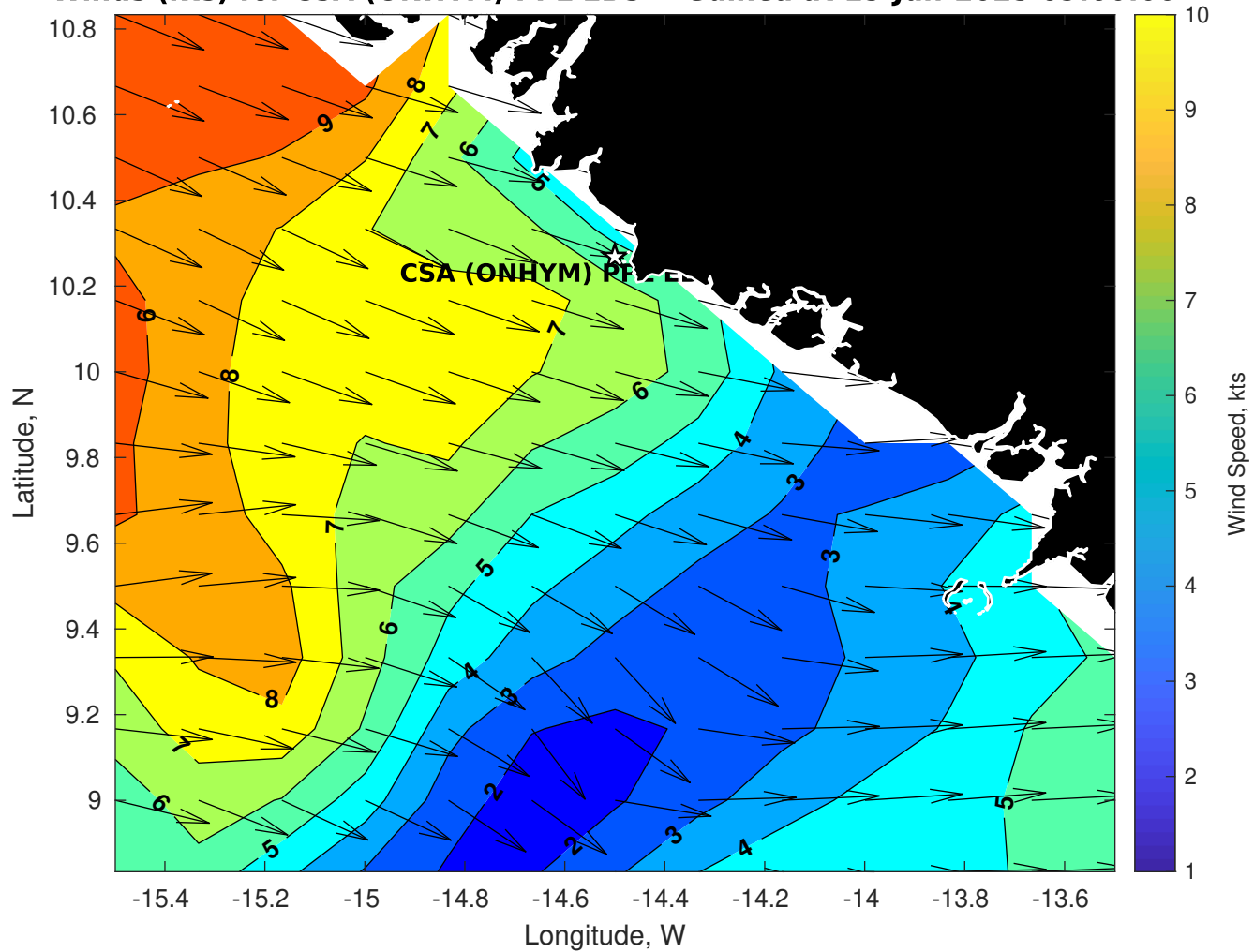
Winds (kts) for CSA (ONHYM) PPL EBS - Guinea at 15-Jun-2025 09:00:00
