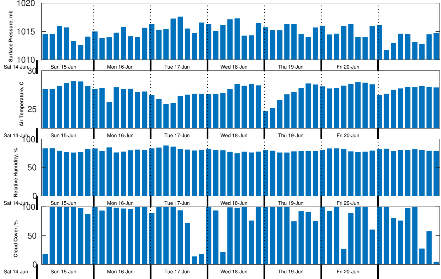
Met Forecast for CSA (ONHYM) PPL EBS - Guinea from 15-Jun-2025 00:00:00 to 22-Jun-2025 00:00:00
