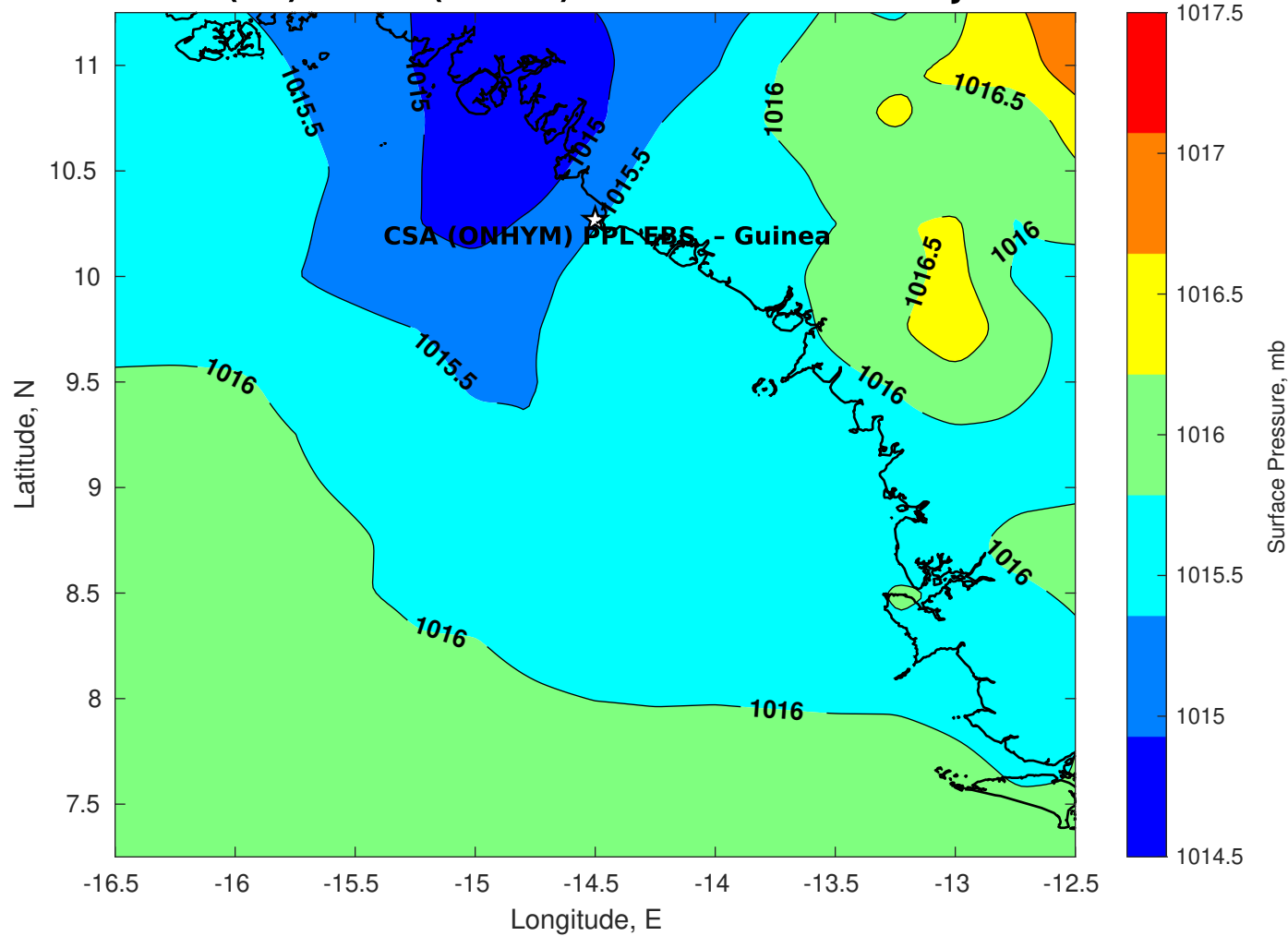
Surface Pressure (mb) for CSA (ONHYM) PPL EBS - Guinea at 15-Jun-2025 00:00:00
