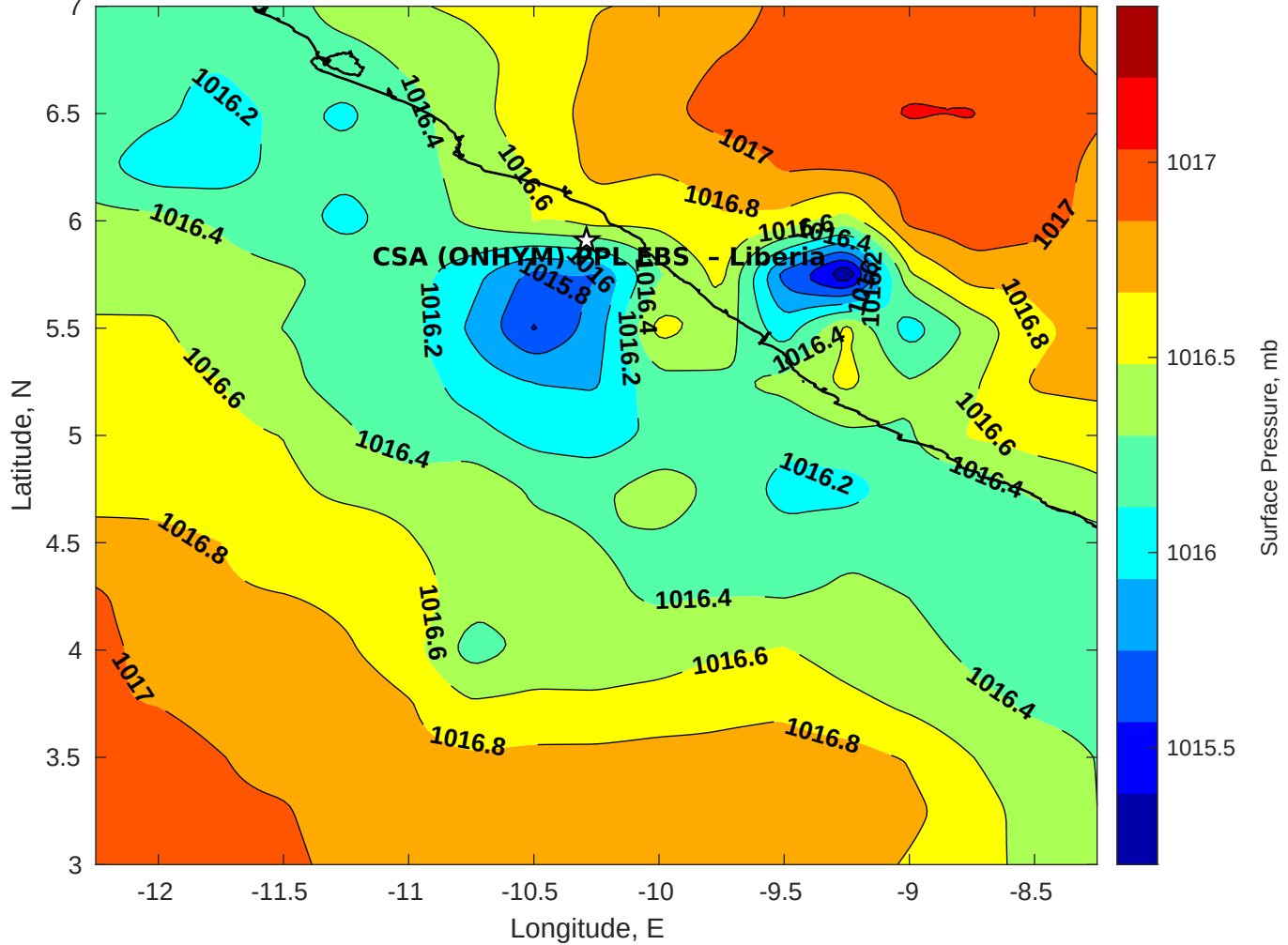
Surface Pressure (mb) for CSA (ONHYM) PPL EBS - Liberia at 15-Jun-2025 00:00:00
