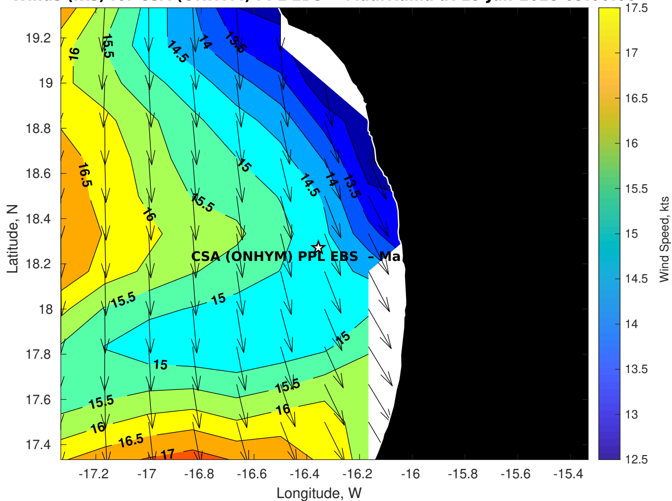
Winds (kts) for CSA (ONHYM) PPL EBS - Mauritania at 15-Jun-2025 09:00:00
