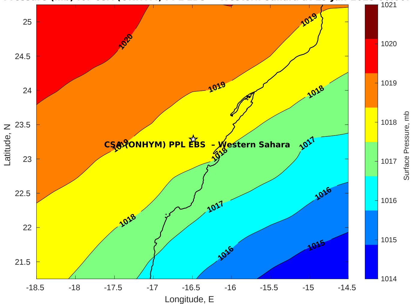
Surface Pressure (mb) for CSA (ONHYM) PPL EBS - Western Sahara at 15-Jun-2025 00:00:00
