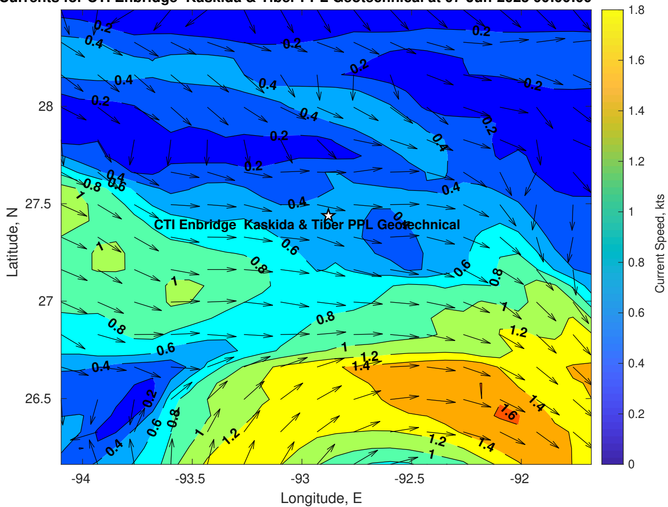
Surface Currents for CTI Enbridge Kaskida & Tiber PPL Geotechnical at 07-Jun-2025 00:00:00
