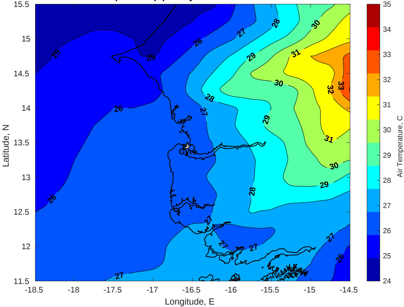
Air Temperature (C) for Gyre at 16-Jun-2025
