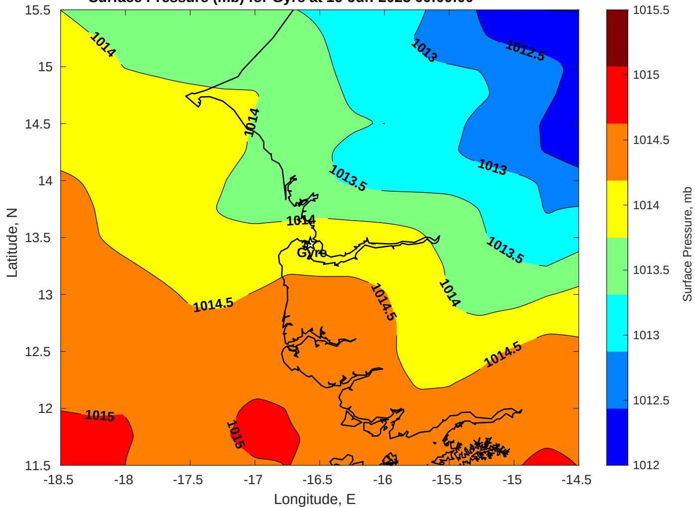
Surface Pressure (mb) for Gyre at 16-Jun-2025 00:00:00
