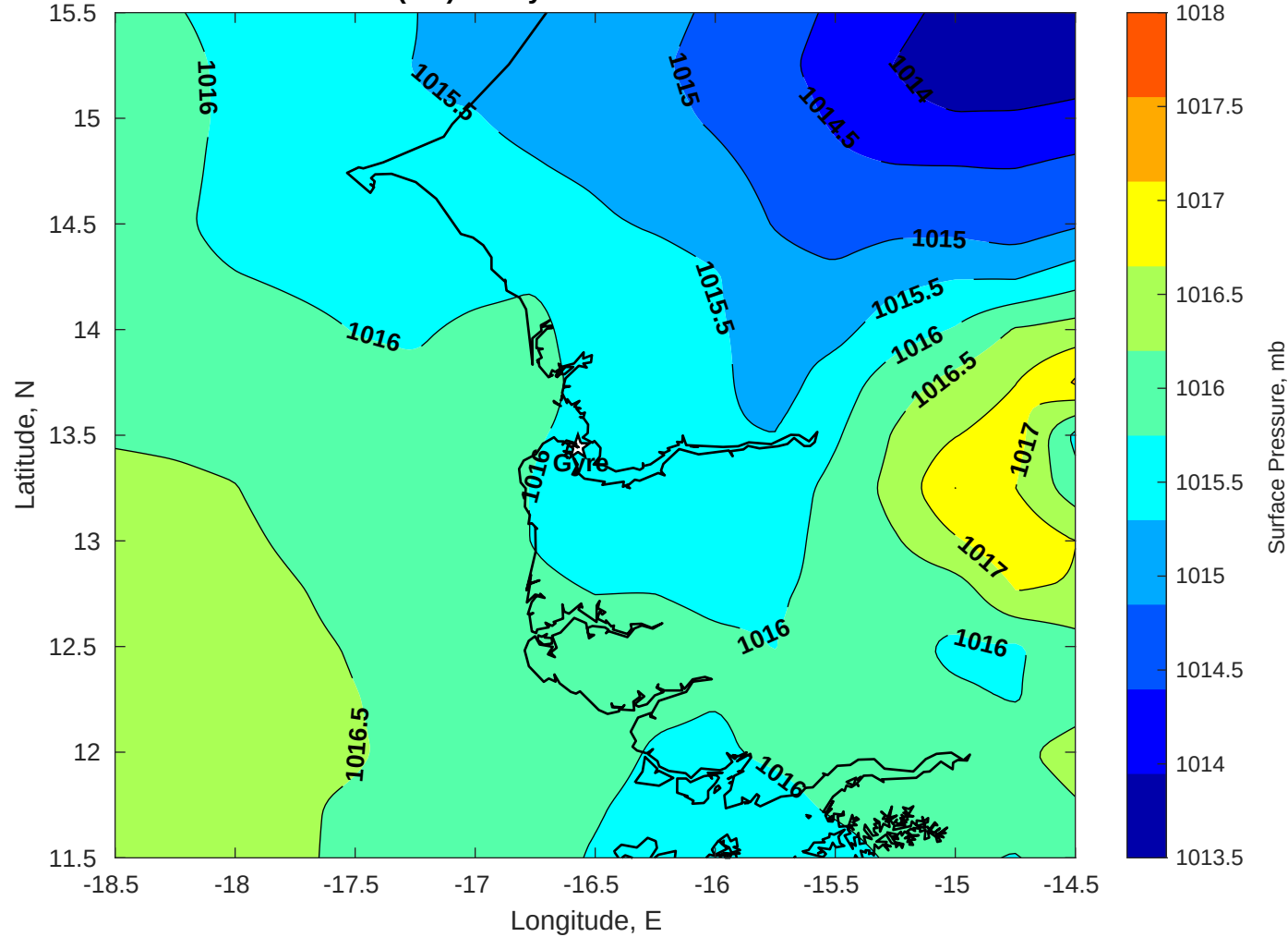
Surface Pressure (mb) for Gyre at 17-Jun-2025 00:00:00
