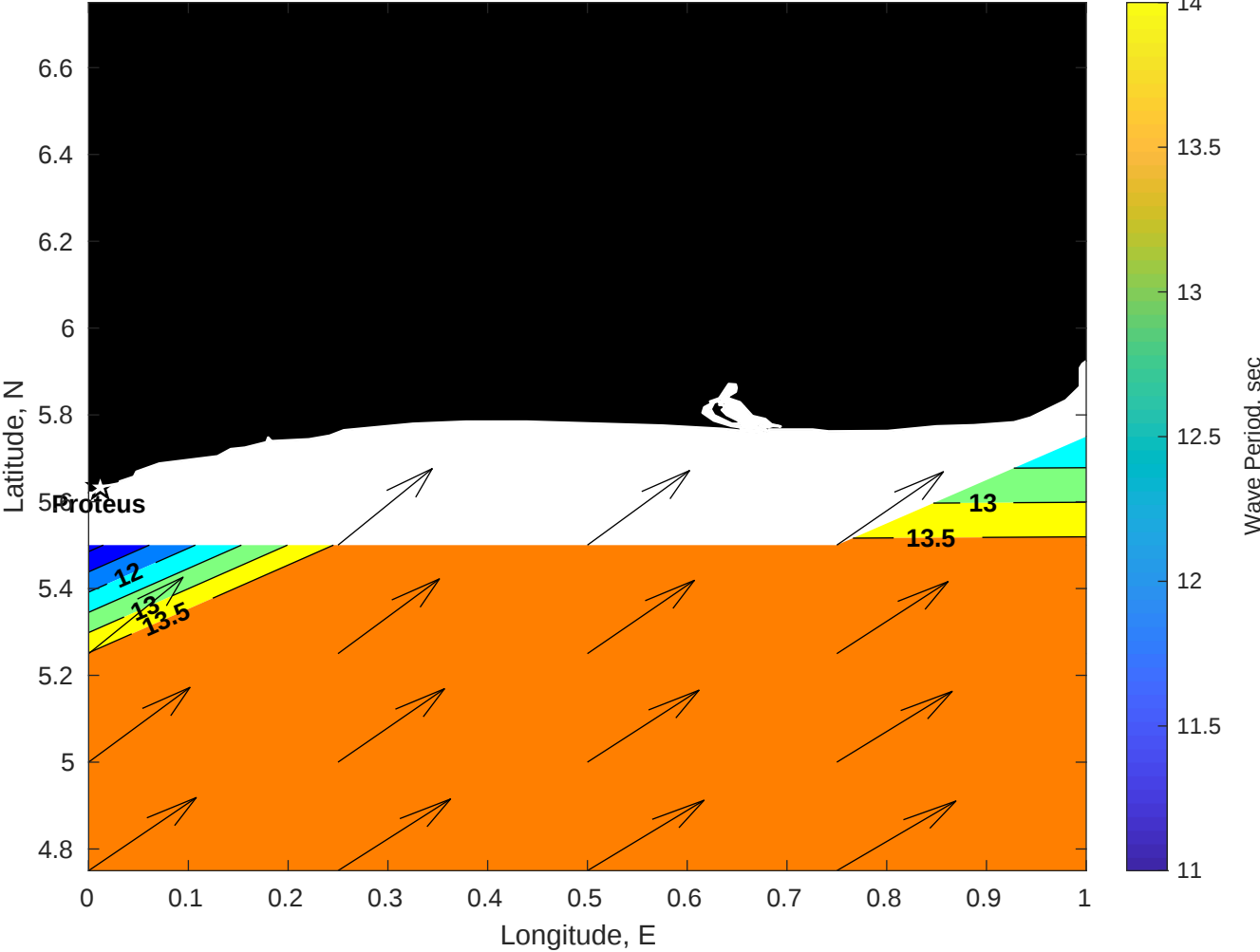
Wave Period (sec) for Proteus at 15-Jun-2025 09:00:00
