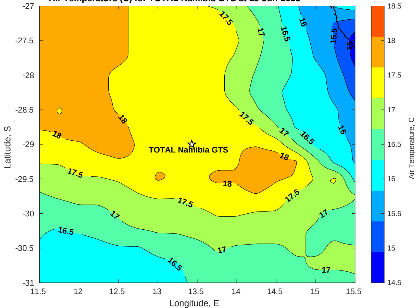
Air Temperature (C) for TOTAL Namibia GTS at 15-Jun-2025
