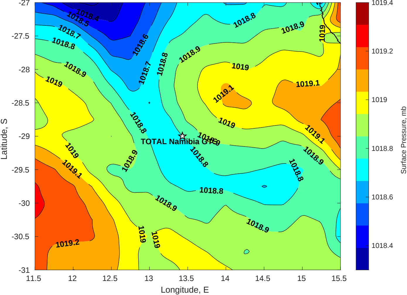
Surface Pressure (mb) for TOTAL Namibia GTS at 15-Jun-2025 00:00:00
