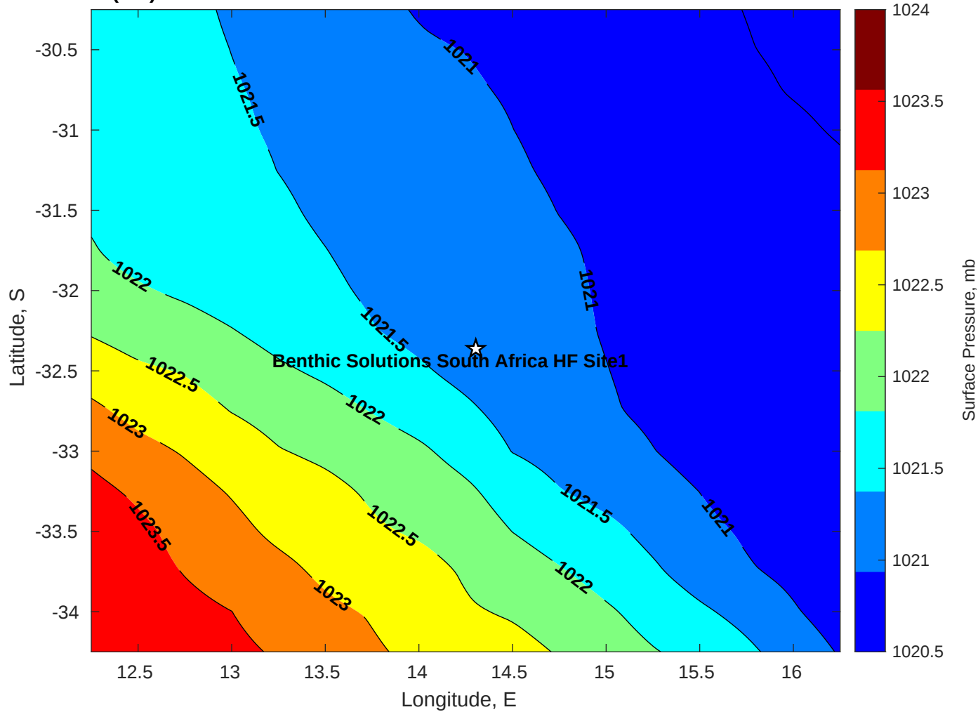
Surface Pressure (mb) for Benthic Solutions South Africa HF Site1 at 16-Jun-2025 00:00:00
