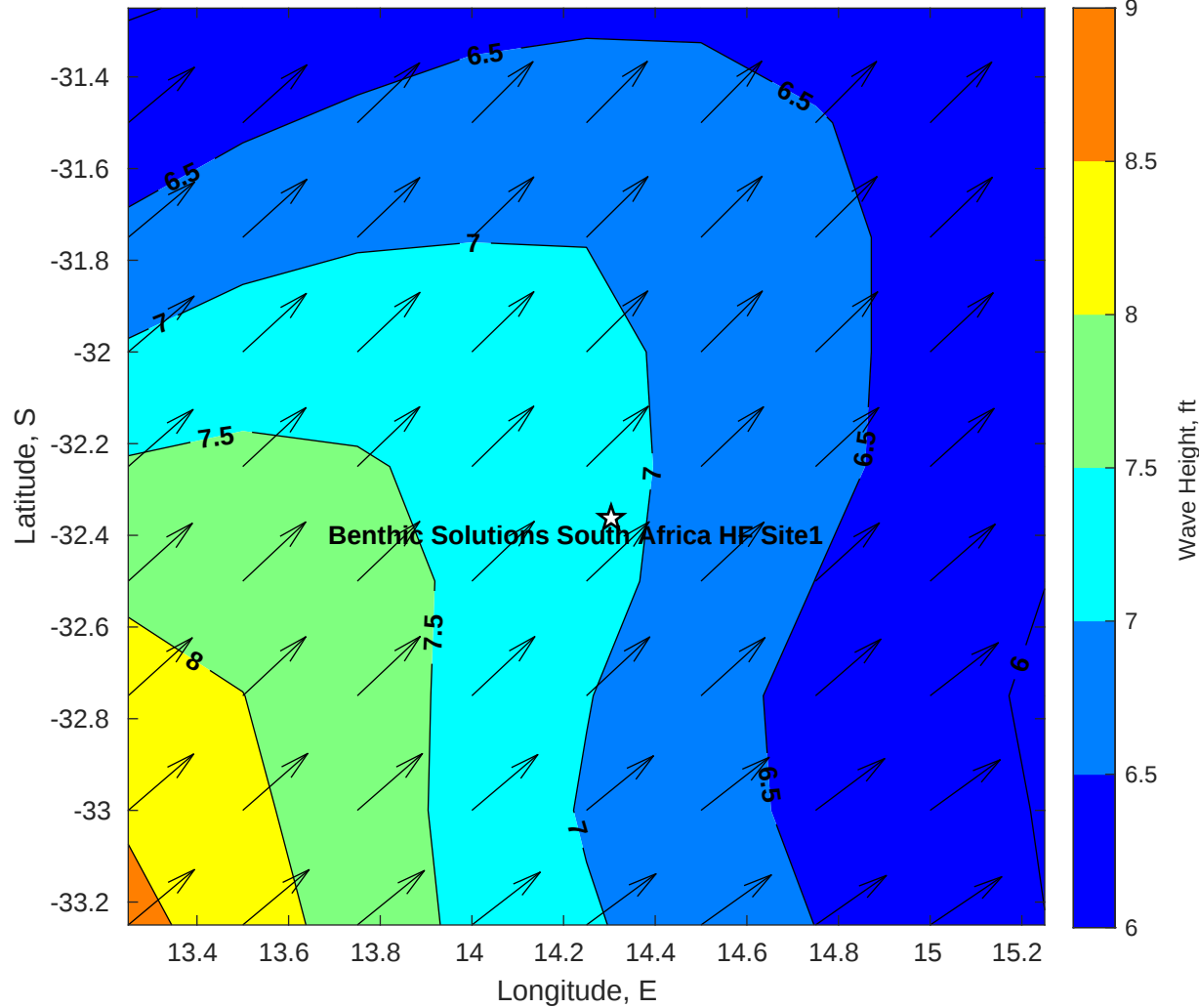
Wave Height (ft) for Benthic Solutions South Africa HF Site1 at 15-Jun-2025 09:00:00
