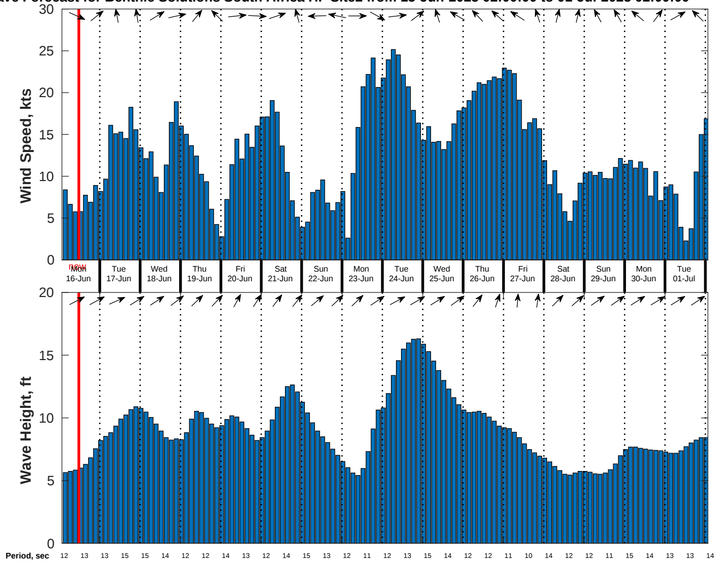
Wind & Wave Forecast for Benthic Solutions South Africa HF Site2 from 15-Jun-2025 02:00:00 to 01-Jul-2025 02:00:00
