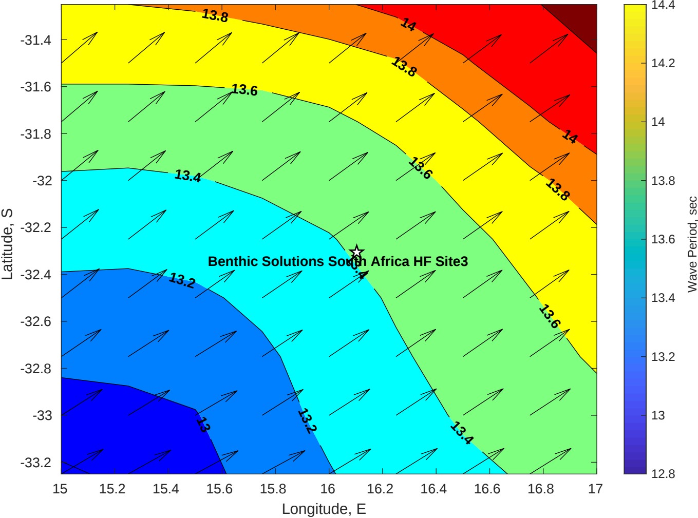
Wave Period (sec) for Benthic Solutions South Africa HF Site3 at 15-Jun-2025 09:00:00
