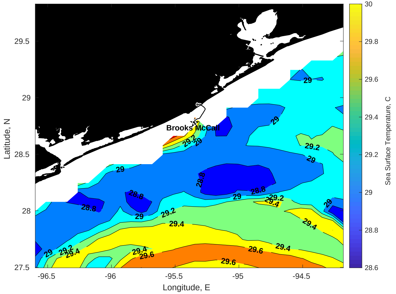
SST for Brooks McCall at 16-Jun-2025 00:00:00
