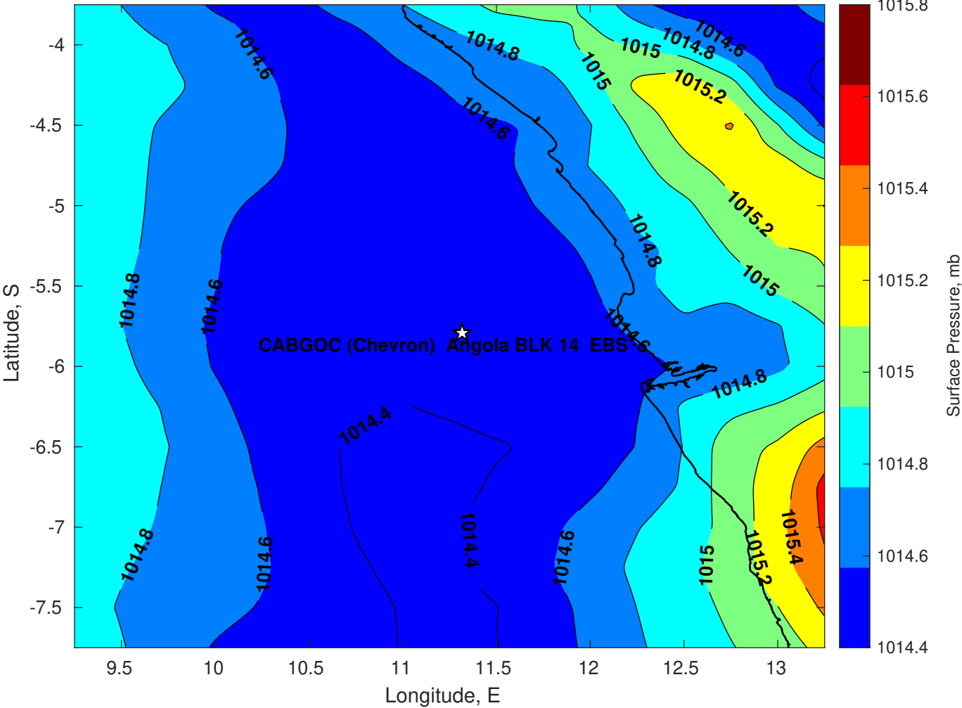
Surface Pressure (mb) for CABGOC (Chevron) Angola BLK 14 EBS at 16-Jun-2025 00:00:00
