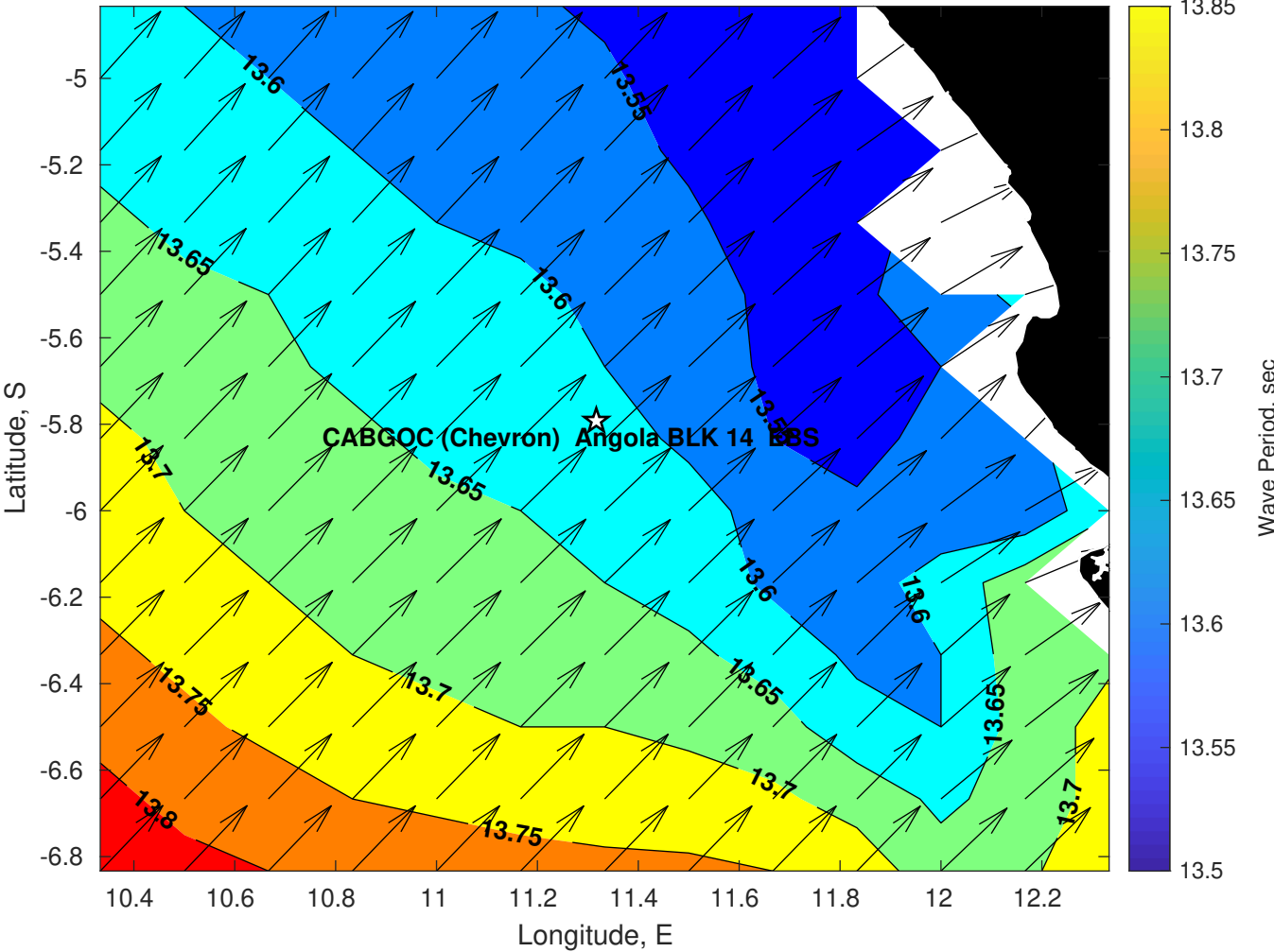
Wave Period (sec) for CABGOC (Chevron) Angola BLK 14 EBS at 15-Jun-2025 09:00:00
