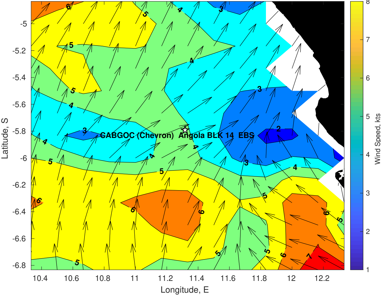
Winds (kts) for CABGOC (Chevron) Angola BLK 14 EBS at 15-Jun-2025 09:00:00
