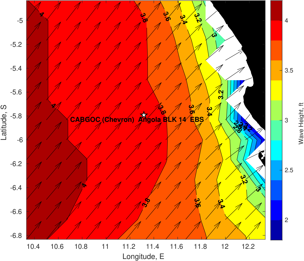
Wave Height (ft) for CABGOC (Chevron) Angola BLK 14 EBS at 15-Jun-2025 09:00:00
