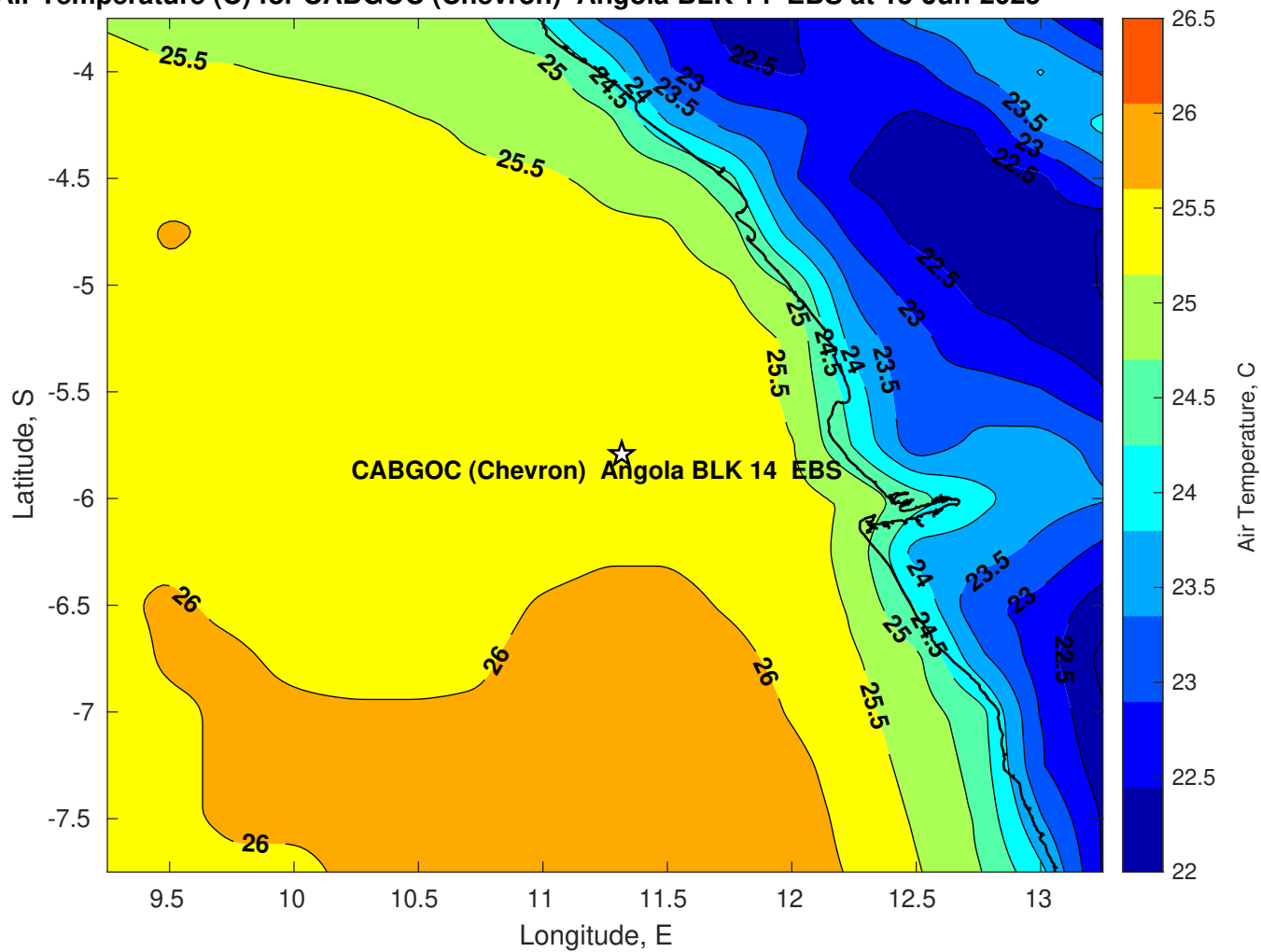
Air Temperature (C) for CABGOC (Chevron) Angola BLK 14 EBS at 15-Jun-2025
