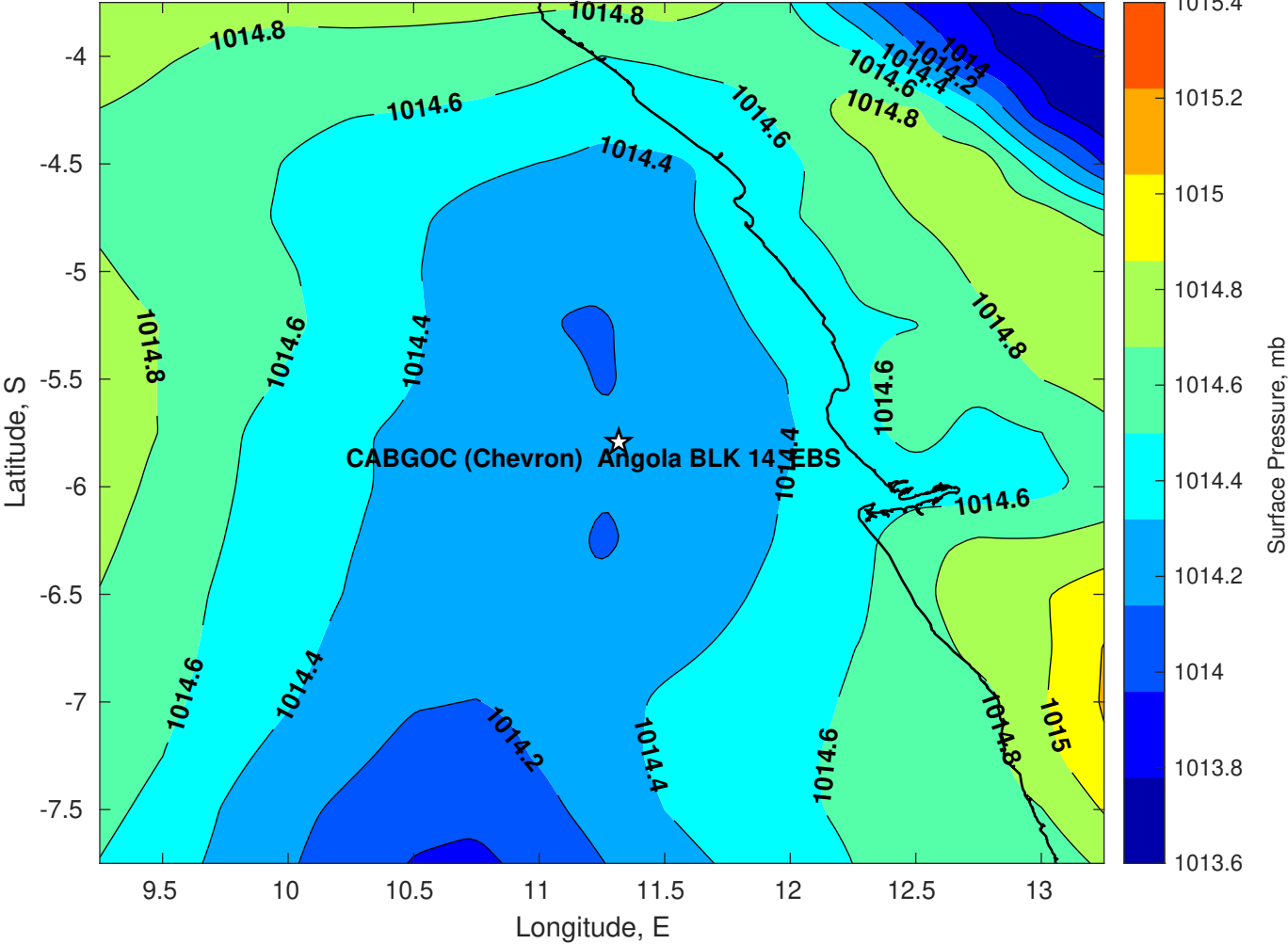
Surface Pressure (mb) for CABGOC (Chevron) Angola BLK 14 EBS at 17-Jun-2025 00:00:00
