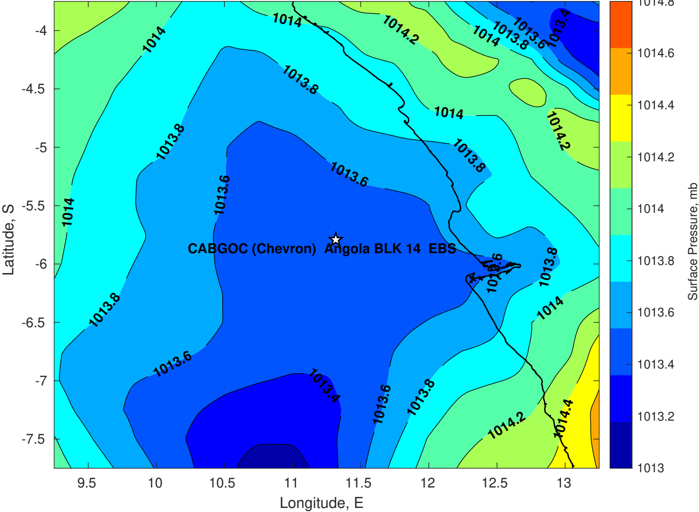
Surface Pressure (mb) for CABGOC (Chevron) Angola BLK 14 EBS at 15-Jun-2025 00:00:00
