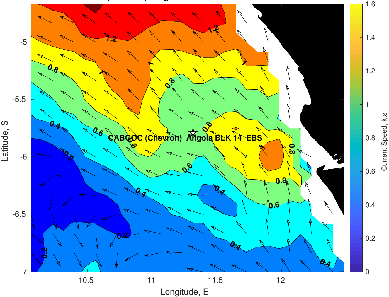
Surface Currents for CABGOC (Chevron) Angola BLK 14 EBS at 07-Jun-2025 00:00:00
