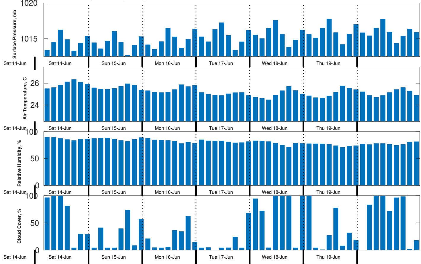
Met Forecast for CABGOC (Chevron) Angola BLK 14 EBS from 15-Jun-2025 00:00:00 to 22-Jun-2025 00:00:00
