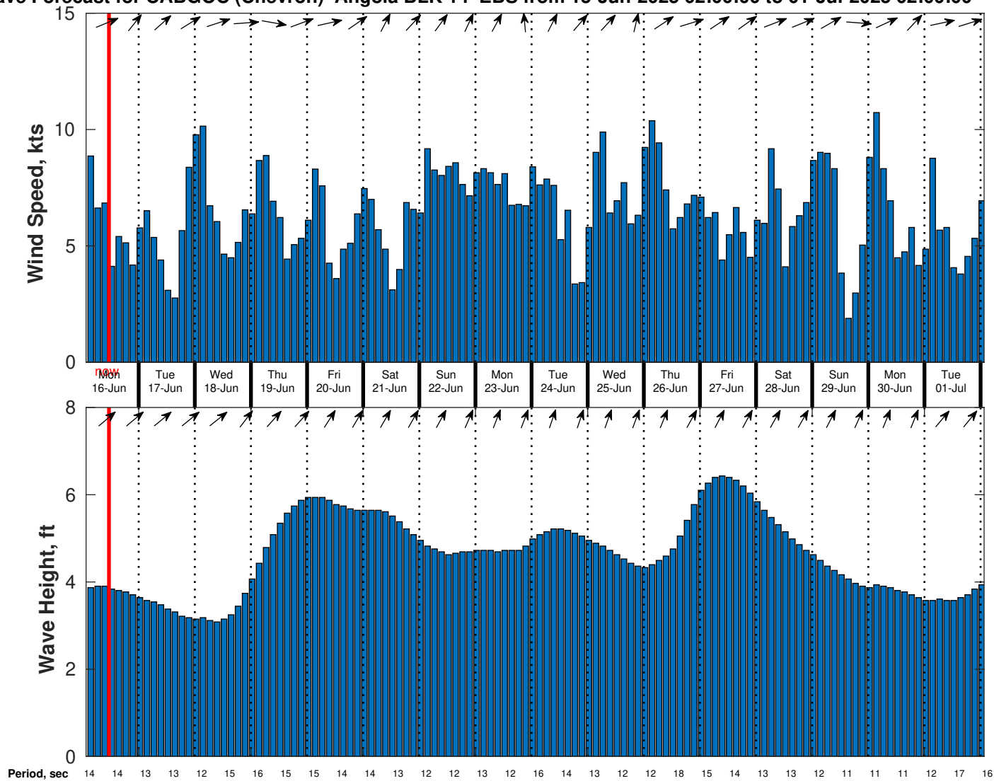
Wind & Wave Forecast for CABGOC (Chevron) Angola BLK 14 EBS from 15-Jun-2025 02:00:00 to 01-Jul-2025 02:00:00
