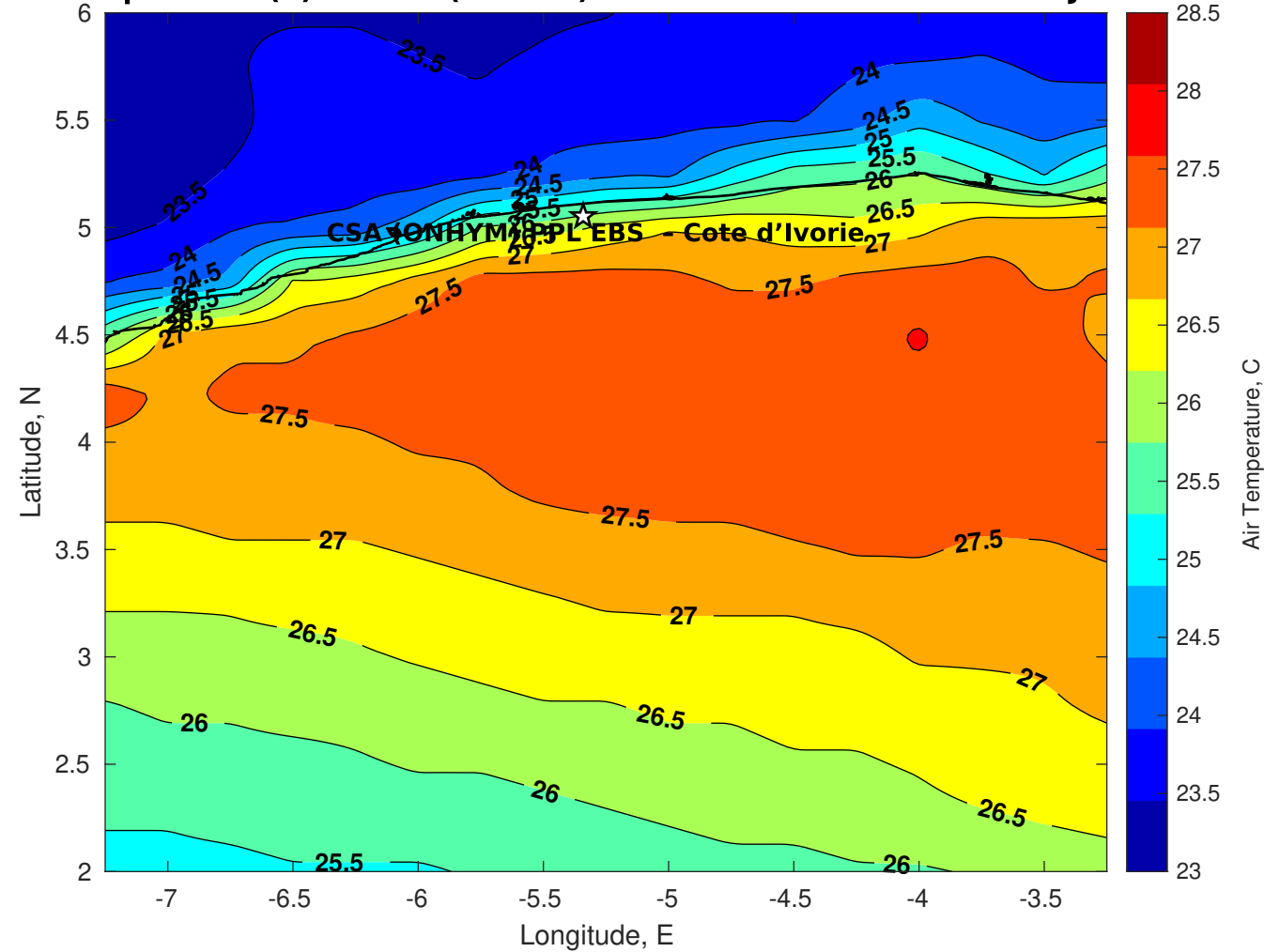
Air Temperature (C) for CSA (ONHYM) PPL EBS - Cote d'Ivoire at 15-Jun-2025
