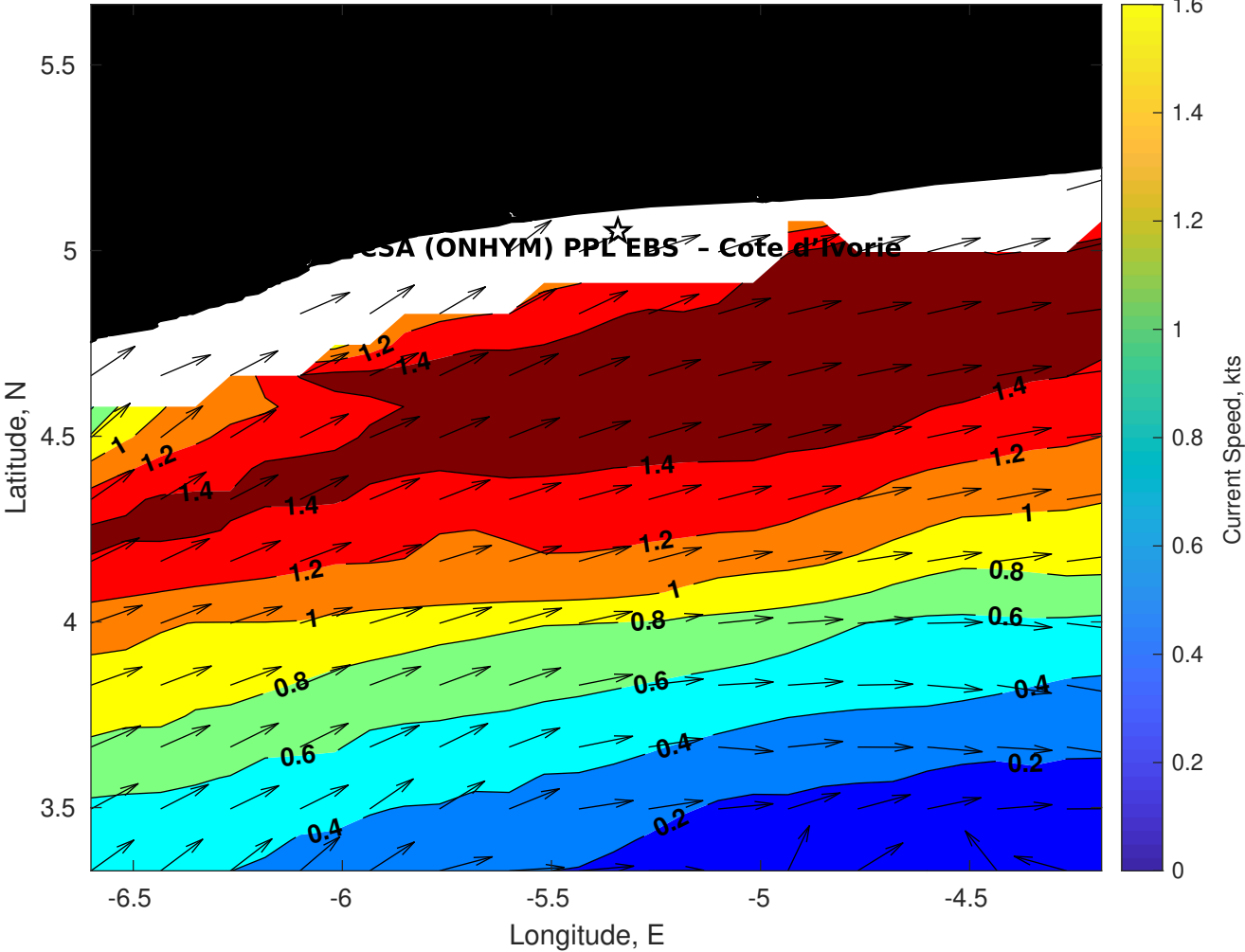
Surface Currents for CSA (ONHYM) PPL EBS - Cote d'Ivoire at 07-Jun-2025 00:00:00
