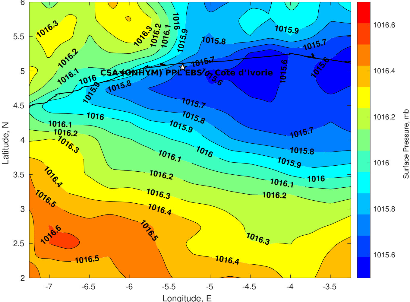
Surface Pressure (mb) for CSA (ONHYM) PPL EBS - Cote d'Ivoire at 16-Jun-2025 00:00:00
