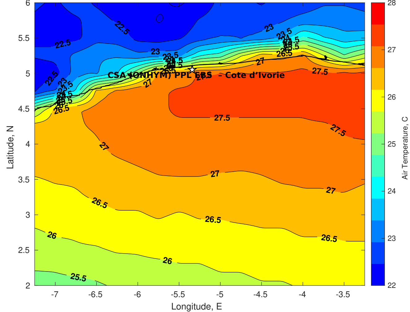
Air Temperature (C) for CSA (ONHYM) PPL EBS - Cote d'Ivoire at 15-Jun-2025
