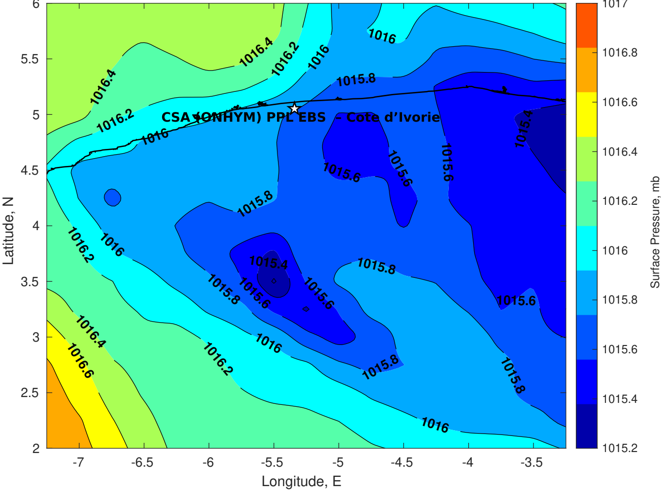
Surface Pressure (mb) for CSA (ONHYM) PPL EBS - Cote d'Ivoire at 17-Jun-2025 00:00:00
