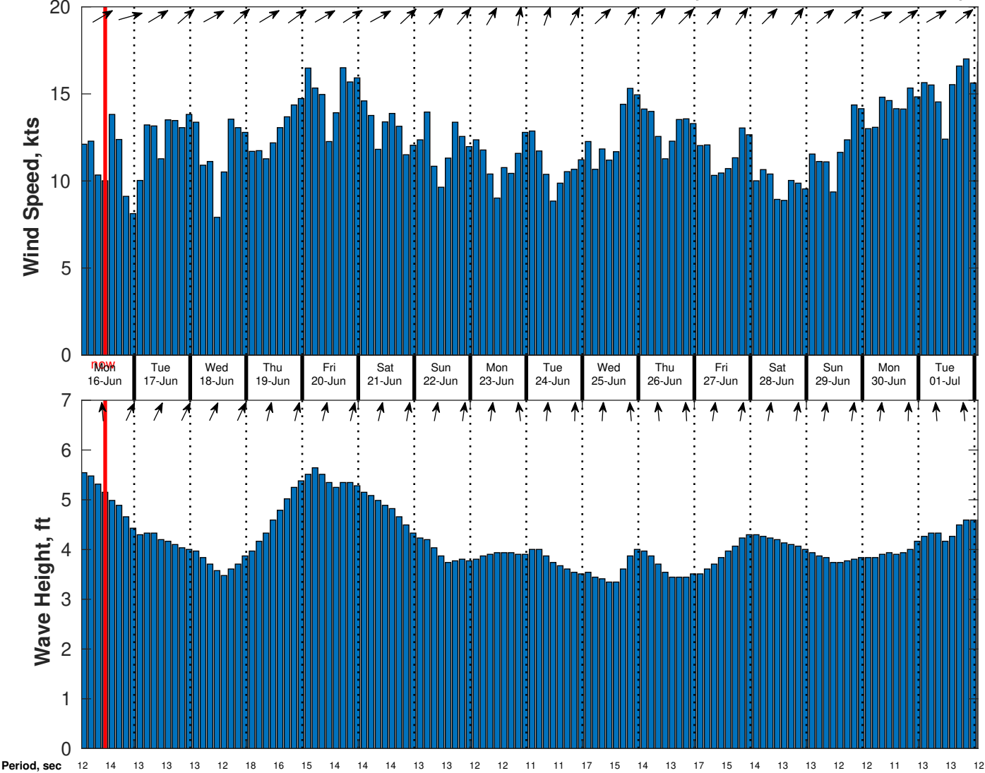
Wind & Wave Forecast for CSA (ONHYM) PPL EBS - Cote d'Ivoire from 15-Jun-2025 01:00:00 to 01-Jul-2025 01:00:00
