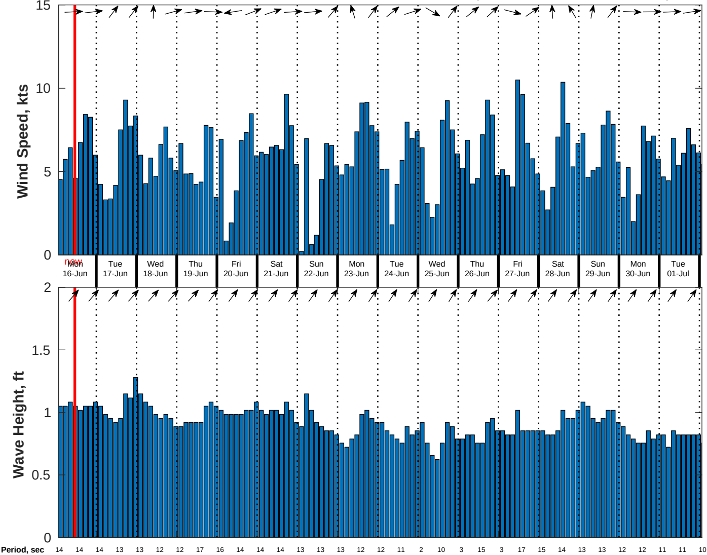
Wind & Wave Forecast for CSA (ONHYM) PPL EBS - Guinea from 15-Jun-2025 01:00:00 to 01-Jul-2025 01:00:00
