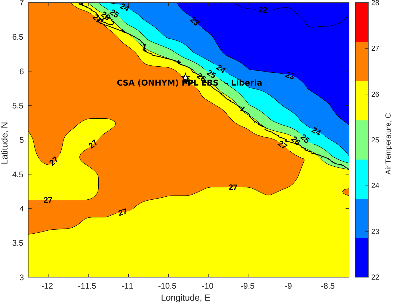
Air Temperature (C) for CSA (ONHYM) PPL EBS - Liberia at 15-Jun-2025
