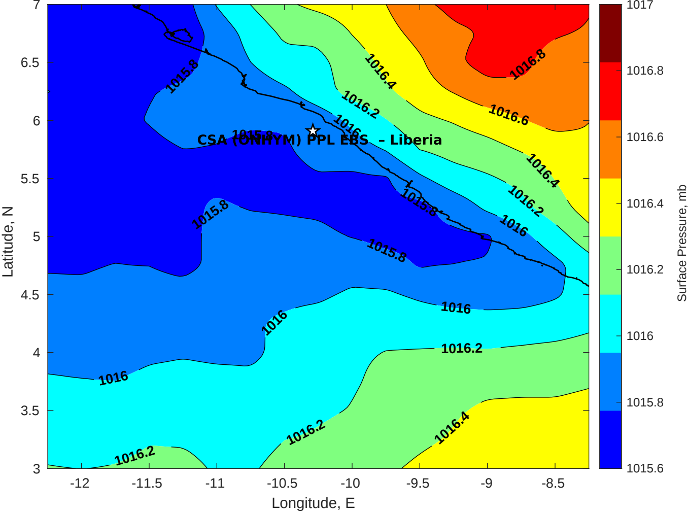
Surface Pressure (mb) for CSA (ONHYM) PPL EBS - Liberia at 16-Jun-2025 00:00:00
