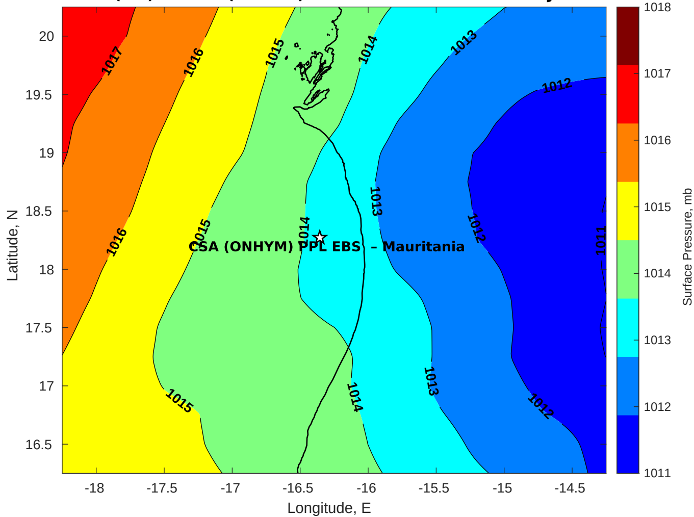
Surface Pressure (mb) for CSA (ONHYM) PPL EBS - Mauritania at 15-Jun-2025 00:00:00
