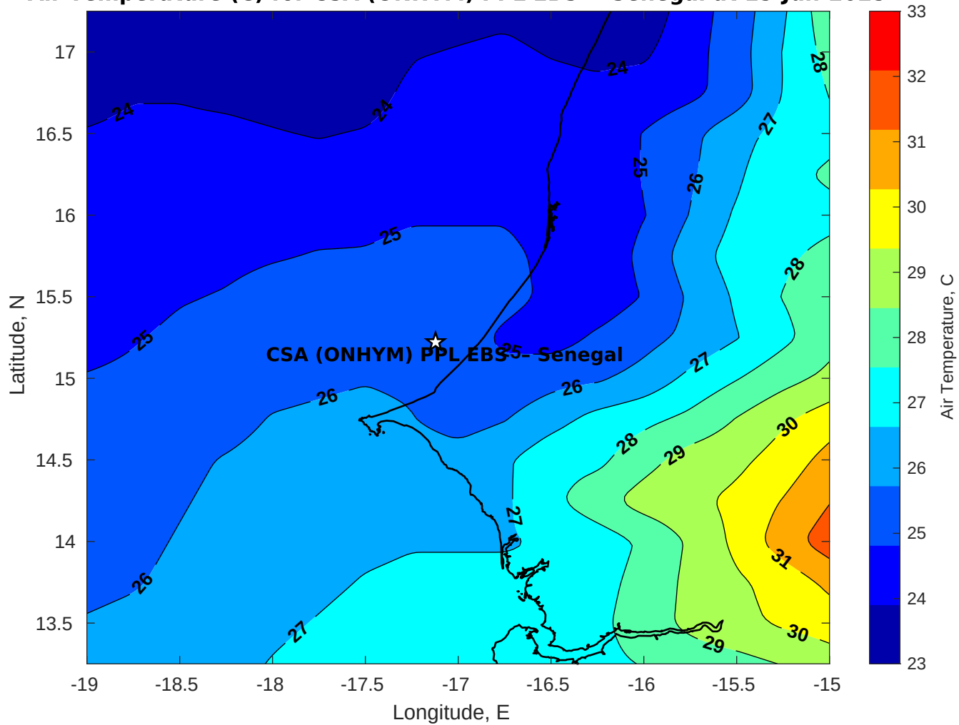
Air Temperature (C) for CSA (ONHYM) PPL EBS - Senegal at 15-Jun-2025
