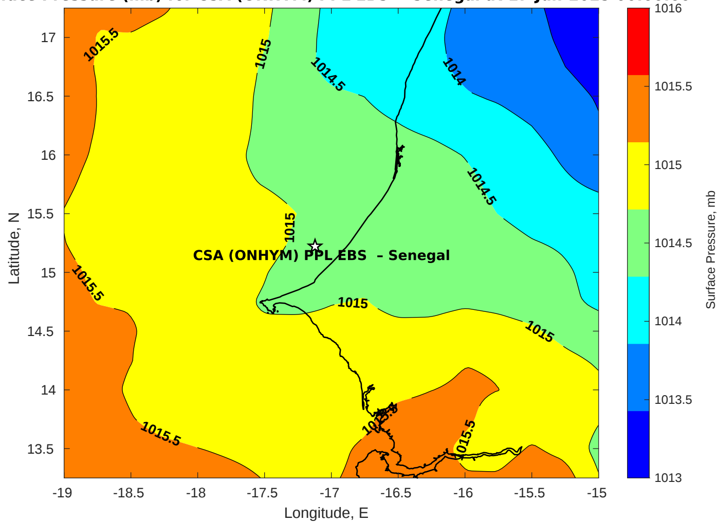
Surface Pressure (mb) for CSA (ONHYM) PPL EBS - Senegal at 17-Jun-2025 00:00:00
