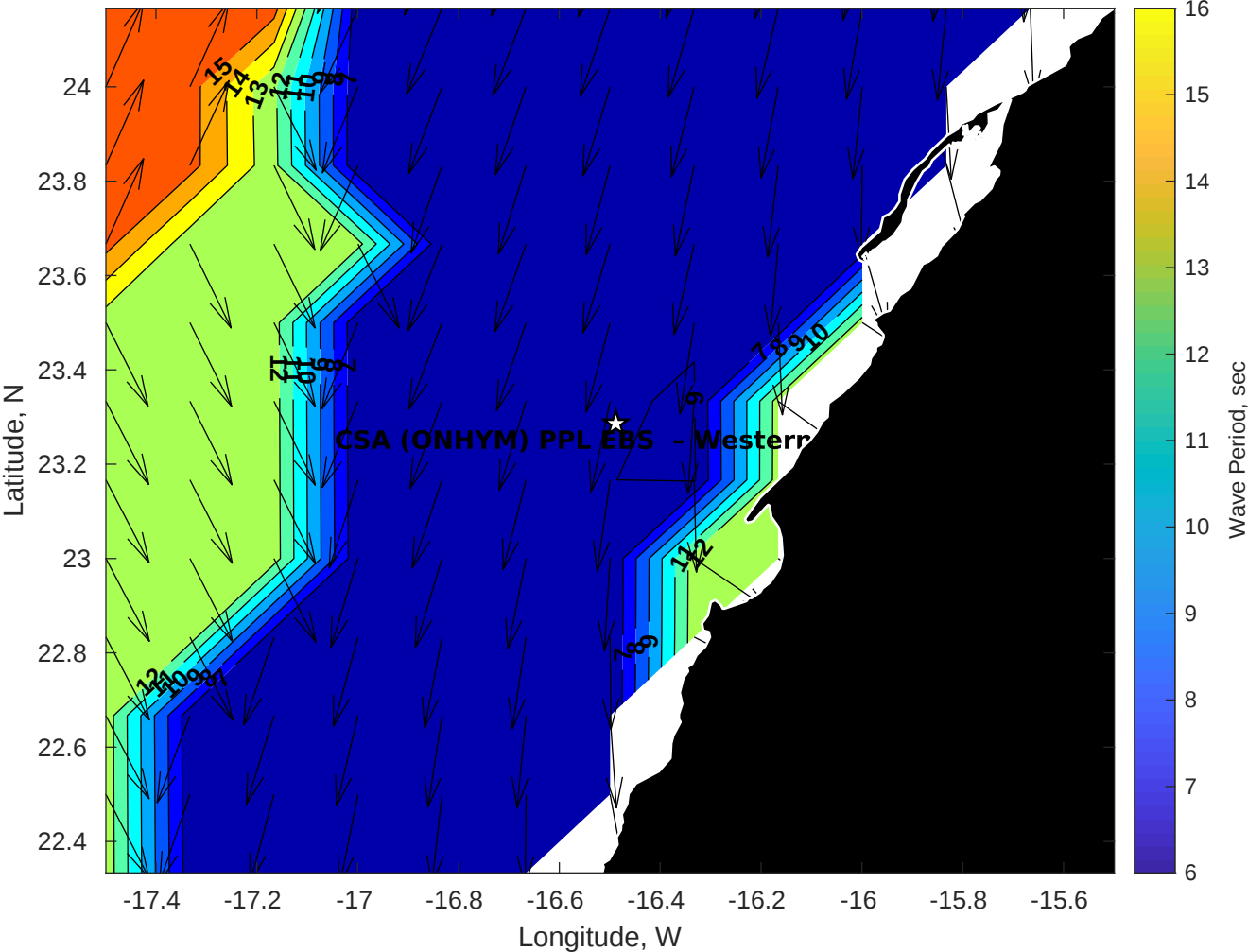
Wave Period (sec) for CSA (ONHYM) PPL EBS - Western Sahara at 15-Jun-2025 09:00:00
