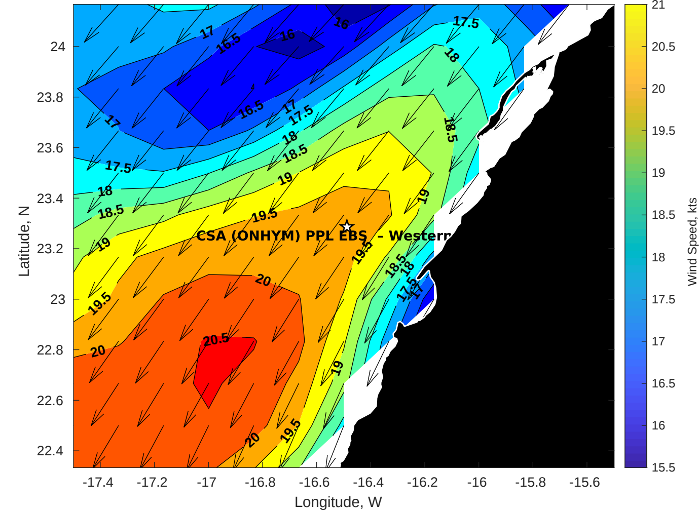
Winds (kts) for CSA (ONHYM) PPL EBS - Western Sahara at 15-Jun-2025 09:00:00
