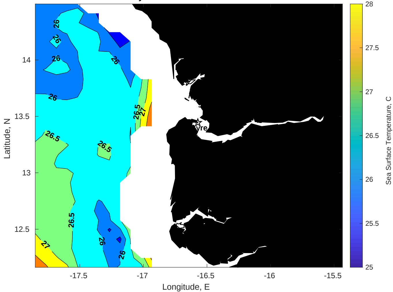
SST for Gyre at 16-Jun-2025 00:00:00
