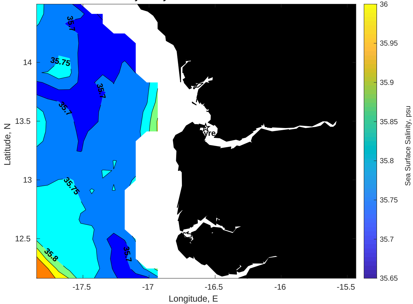
Surface Salinity for Gyre at 16-Jun-2025 00:00:00
