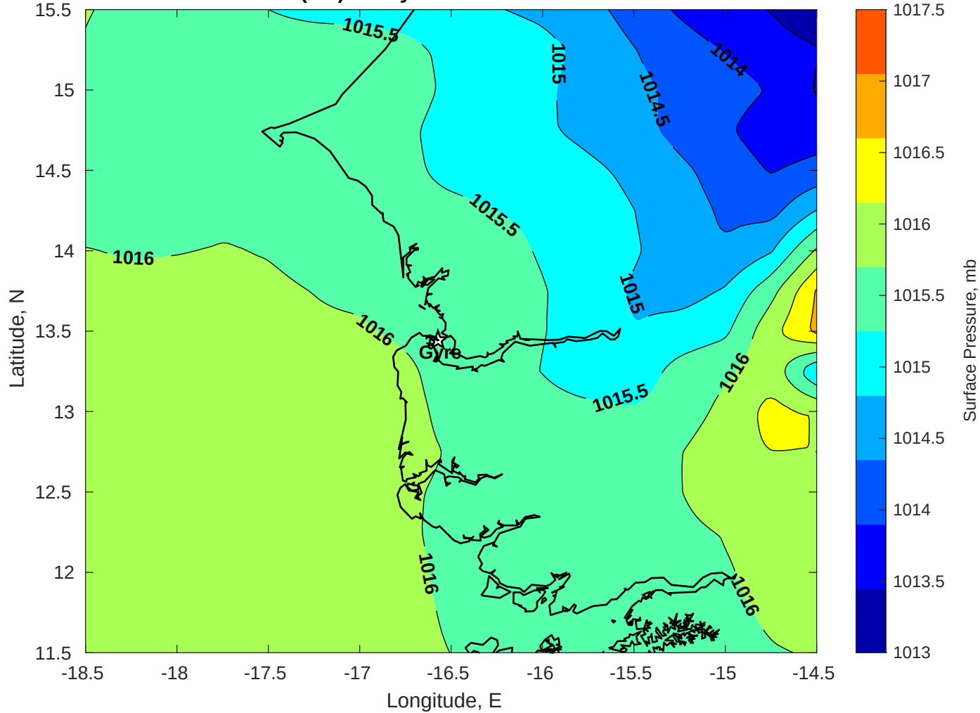
Surface Pressure (mb) for Gyre at 17-Jun-2025 00:00:00
