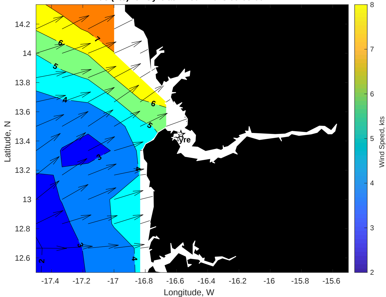
Winds (kts) for Gyre at 17-Jun-2025 09:00:00
