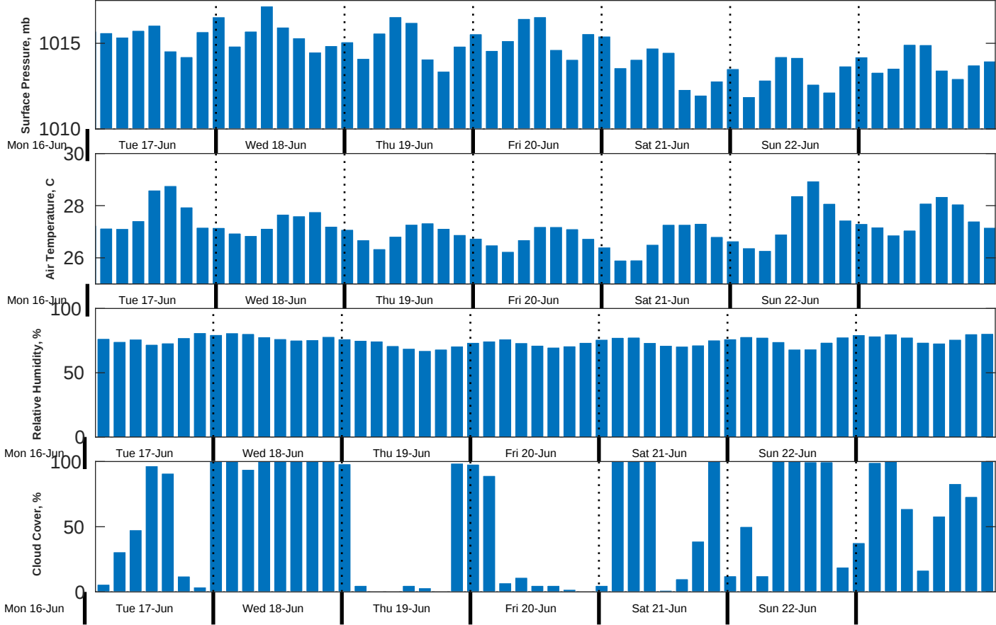
Met Forecast for Gyre from 16-Jun-2025 23:00:00 to 23-Jun-2025 23:00:00
