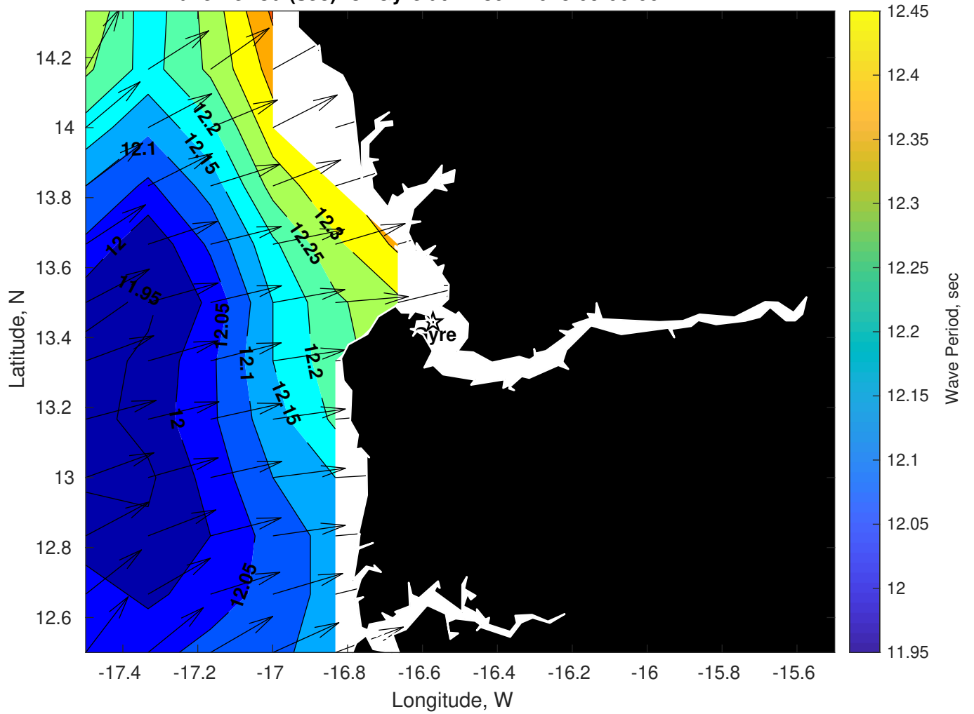
Wave Period (sec) for Gyre at 17-Jun-2025 09:00:00
