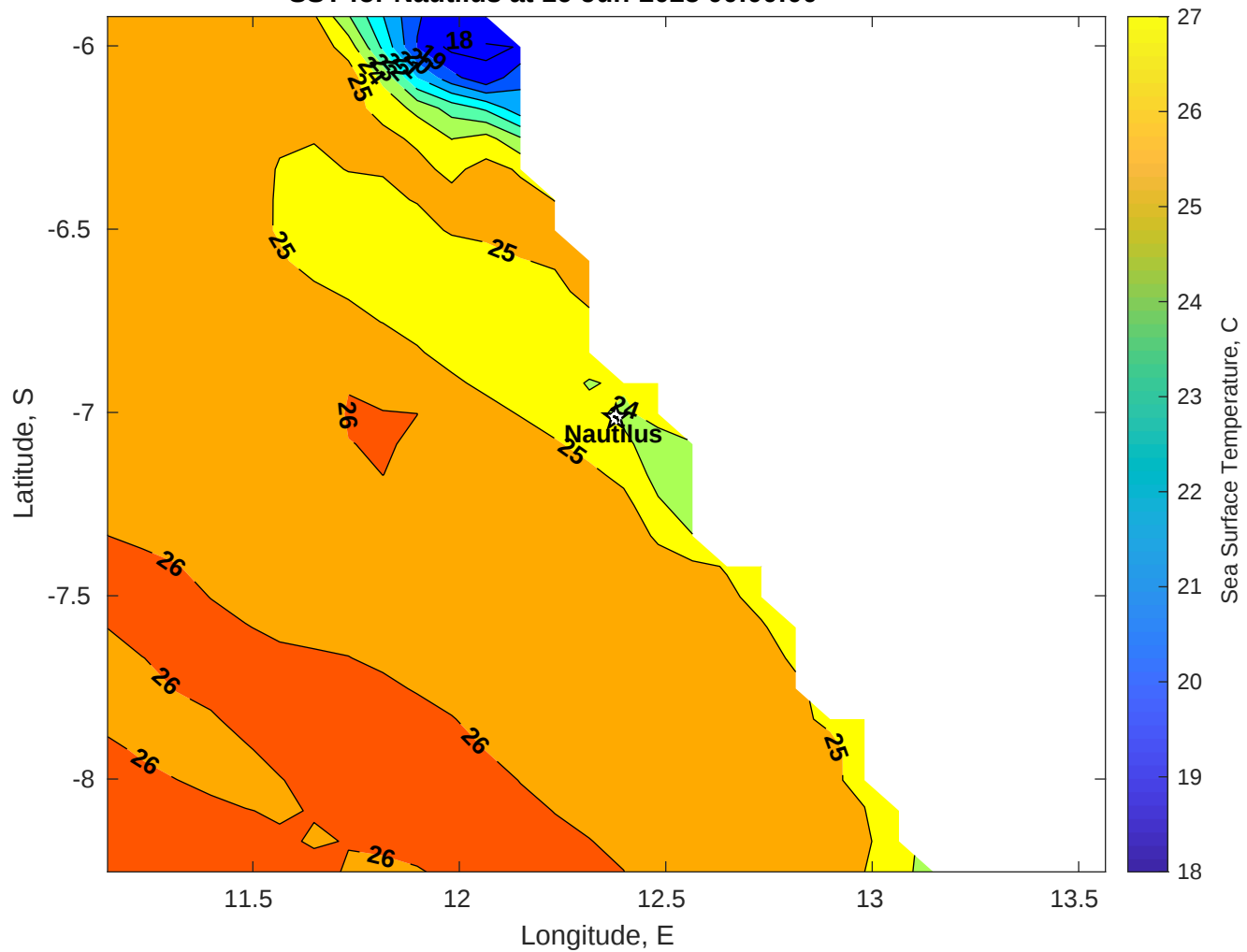
SST for Nautilus at 16-Jun-2025 00:00:00
