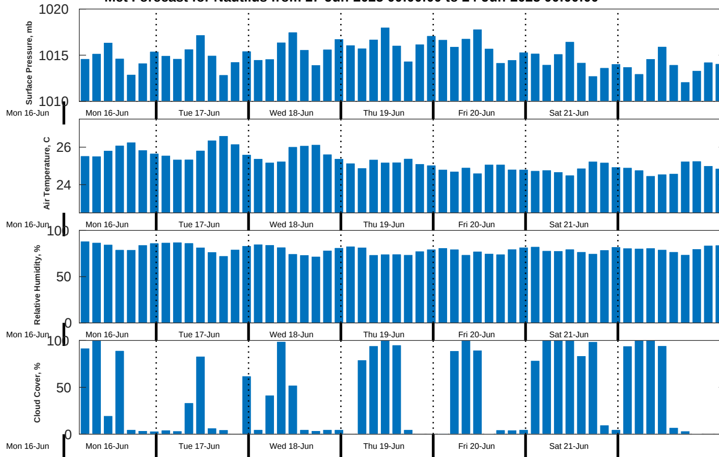
Met Forecast for Nautilus from 17-Jun-2025 00:00:00 to 24-Jun-2025 00:00:00
