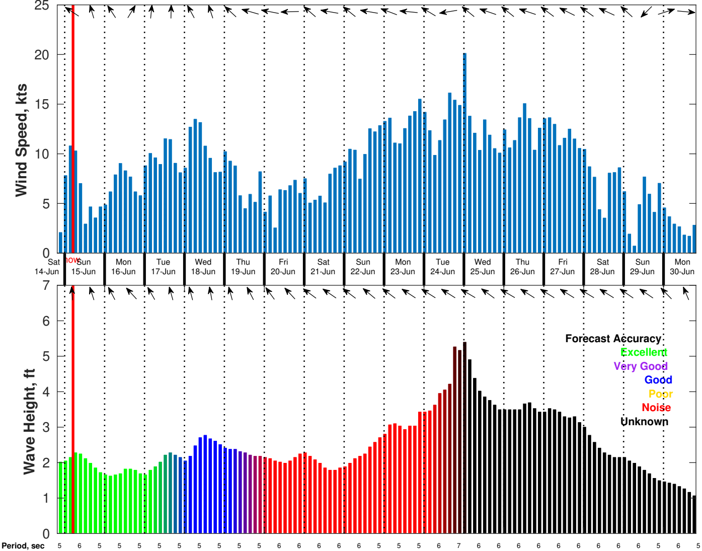
Wind & Wave Forecast for Shell Noches GC19 PPL Geotechnical from 14-Jun-2025 20:00:00 to 30-Jun-2025 20:00:00
