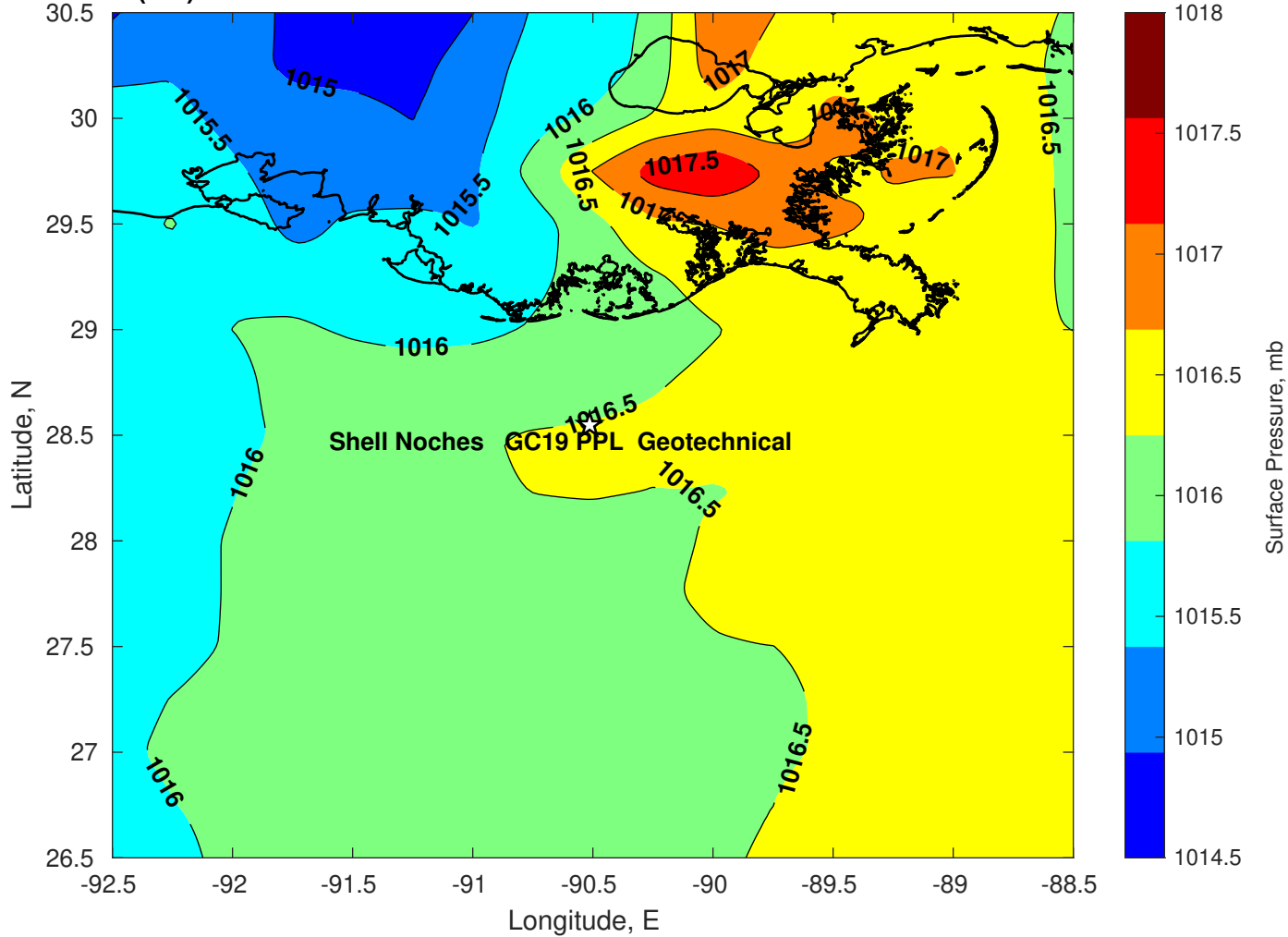
Surface Pressure (mb) for Shell Noches GC19 PPL Geotechnical at 16-Jun-2025 00:00:00
