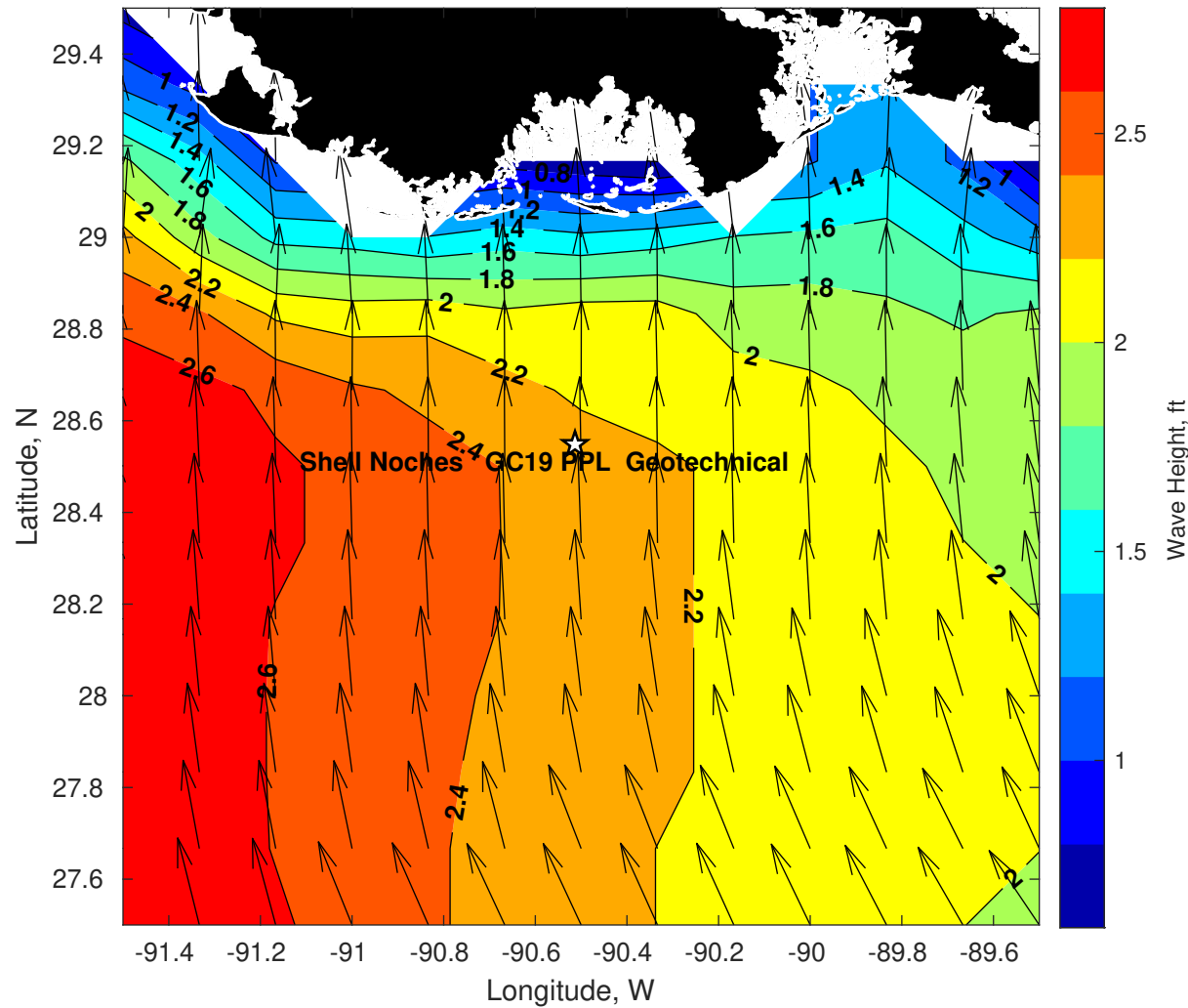
Wave Height (ft) for Shell Noches GC19 PPL Geotechnical at 15-Jun-2025 09:00:00
