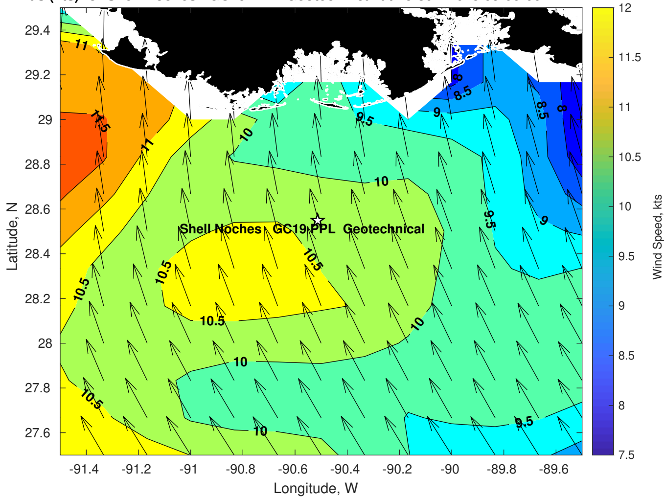
Winds (kts) for Shell Noches GC19 PPL Geotechnical at 15-Jun-2025 09:00:00
