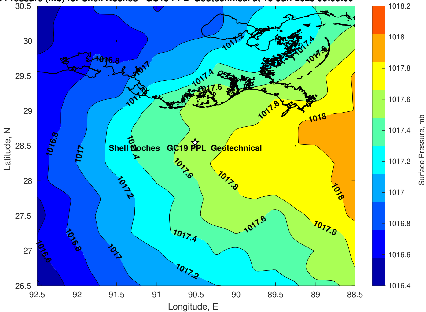
Surface Pressure (mb) for Shell Noches GC19 PPL Geotechnical at 15-Jun-2025 00:00:00
