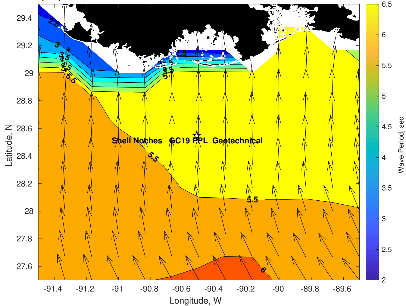
Wave Period (sec) for Shell Noches GC19 PPL Geotechnical at 15-Jun-2025 09:00:00
