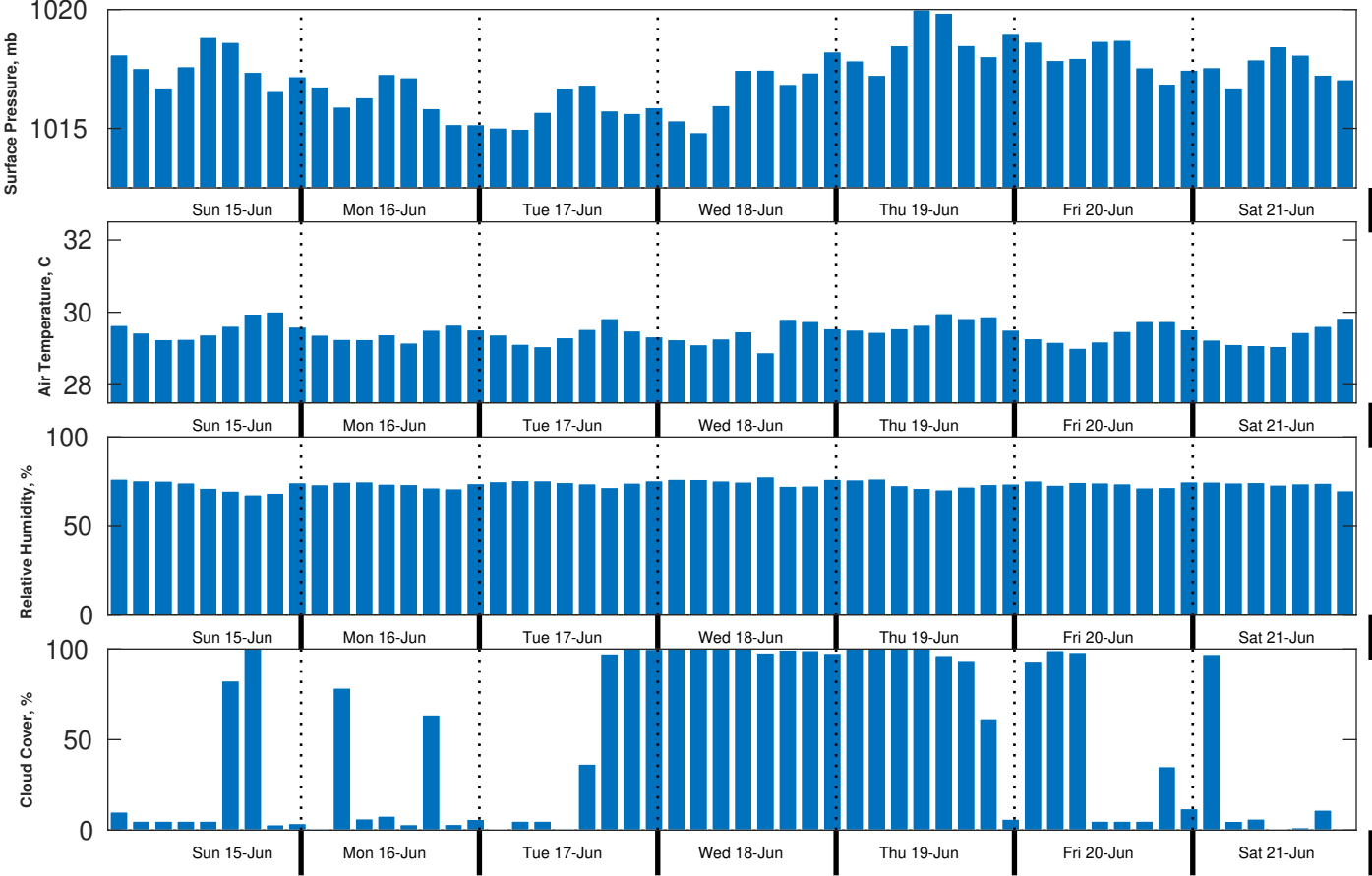
Met Forecast for Shell Noches GC19 PPL Geotechnical from 15-Jun-2025 00:00:00 to 22-Jun-2025 00:00:00
