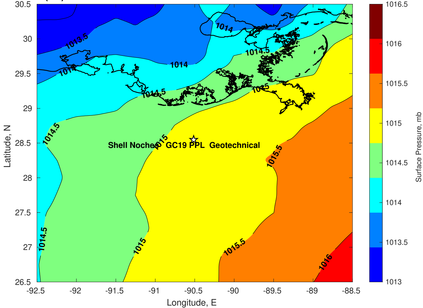
Surface Pressure (mb) for Shell Noches GC19 PPL Geotechnical at 17-Jun-2025 00:00:00
