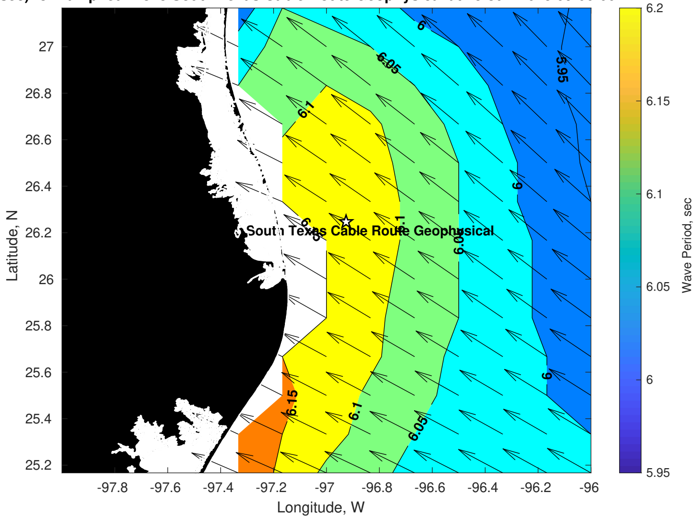
Period (sec) for Tampnet P2378 South Texas Cable Route Geophysical at 15-Jun-2025 09:00:00
