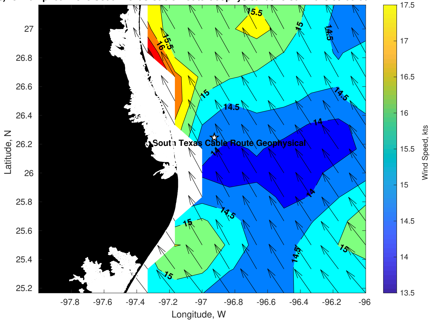
Winds (kts) for Tampnet P2378 South Texas Cable Route Geophysical at 15-Jun-2025 09:00:00
