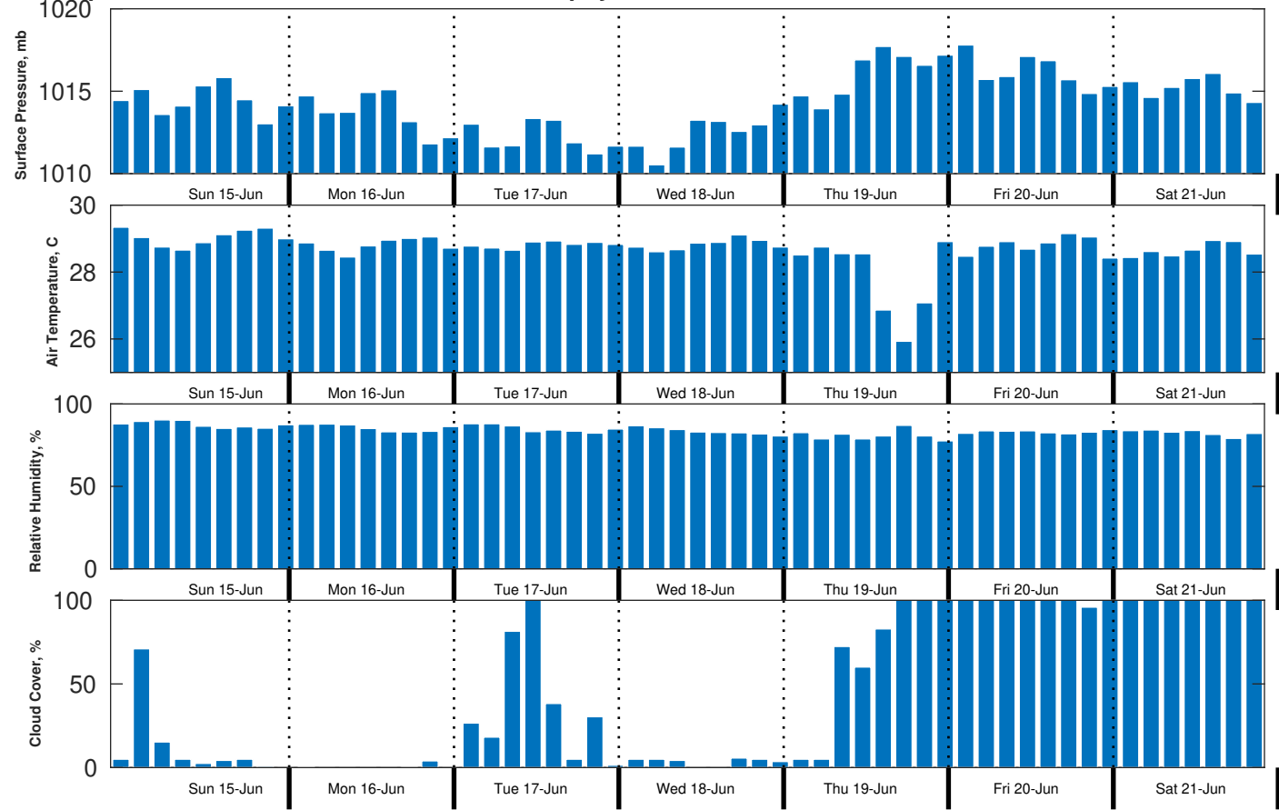
Met Forecast for Tampnet P2378 South Texas Cable Route Geophysical from 15-Jun-2025 00:00:00 to 22-Jun-2025 00:00:00
