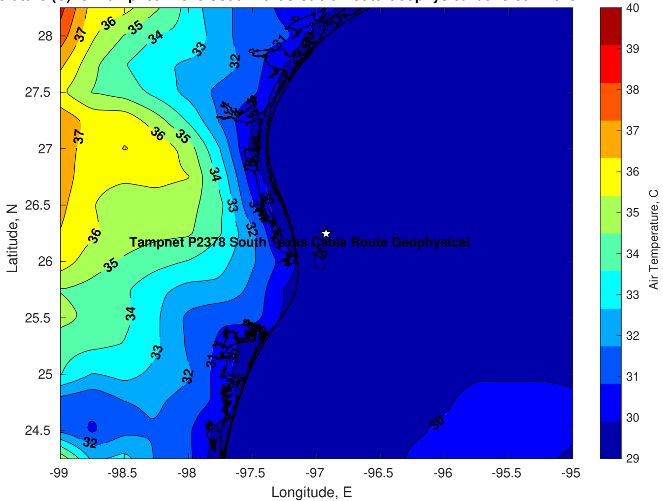
Air Temperature (C) for Tampnet P2378 South Texas Cable Route Geophysical at 15-Jun-2025
