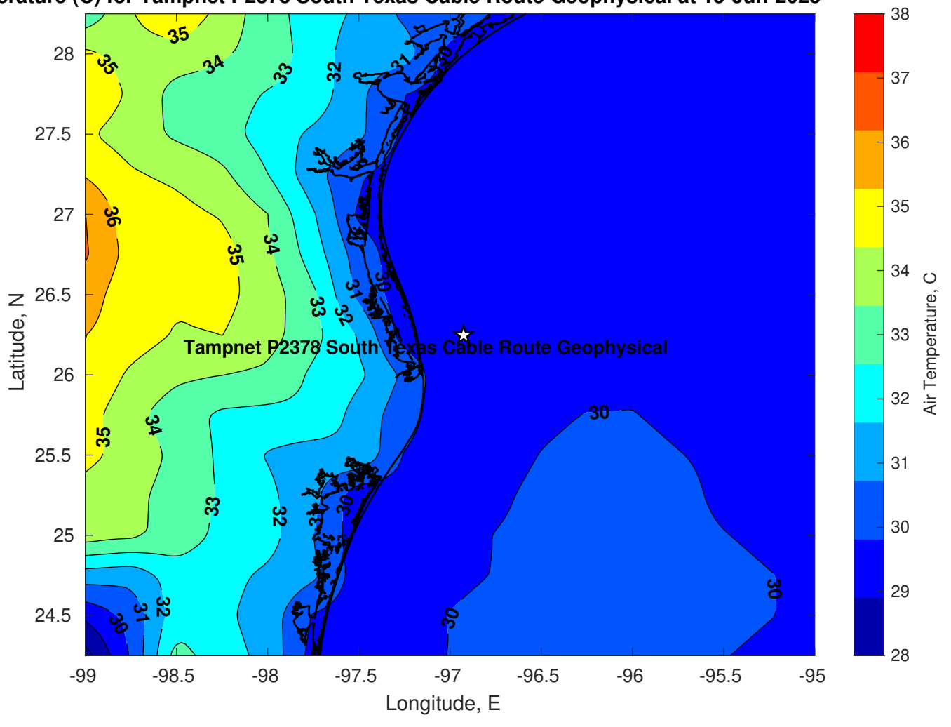
Air Temperature (C) for Tampnet P2378 South Texas Cable Route Geophysical at 15-Jun-2025
