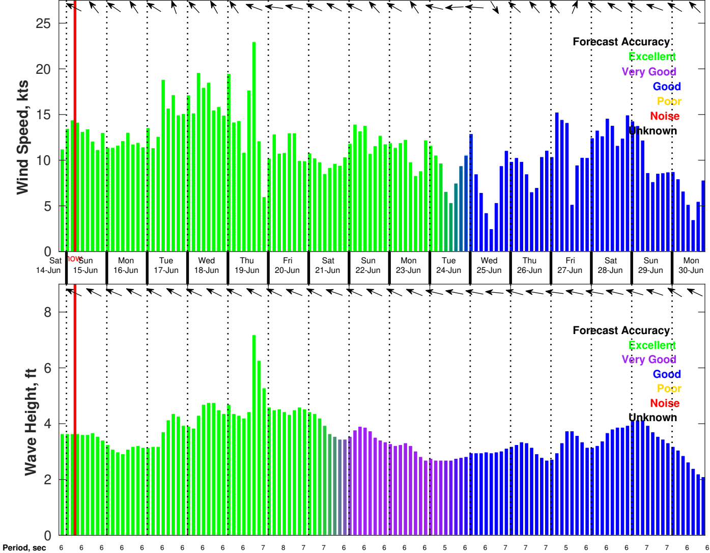
Wind & Wave Forecast for Tampnet P2378 South Texas Cable Route Geophysical from 14-Jun-2025 20:00:00 to 30-Jun-2025 20:00:00
