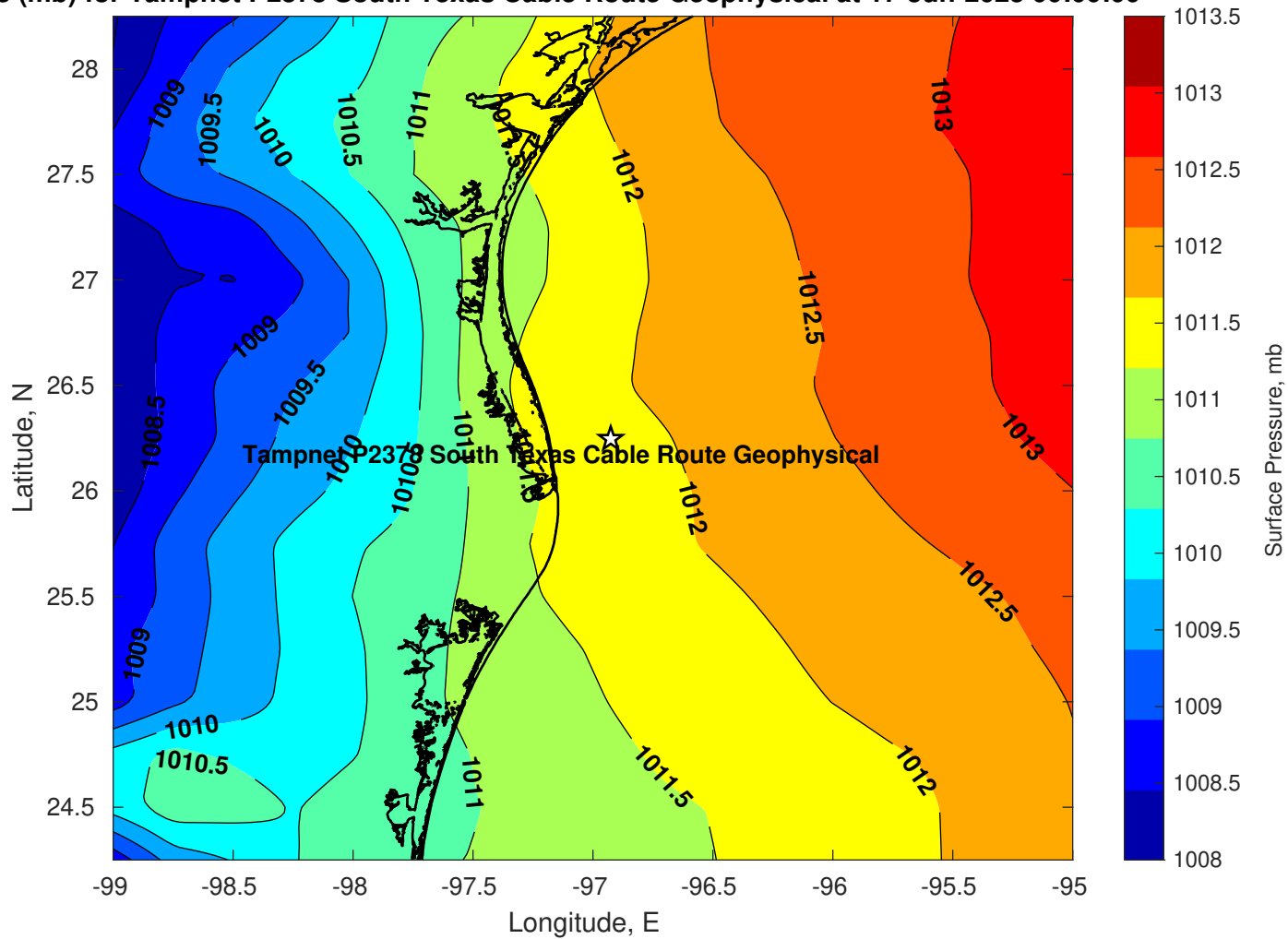
Pressure (mb) for Tampnet P2378 South Texas Cable Route Geophysical at 17-Jun-2025 00:00:00
