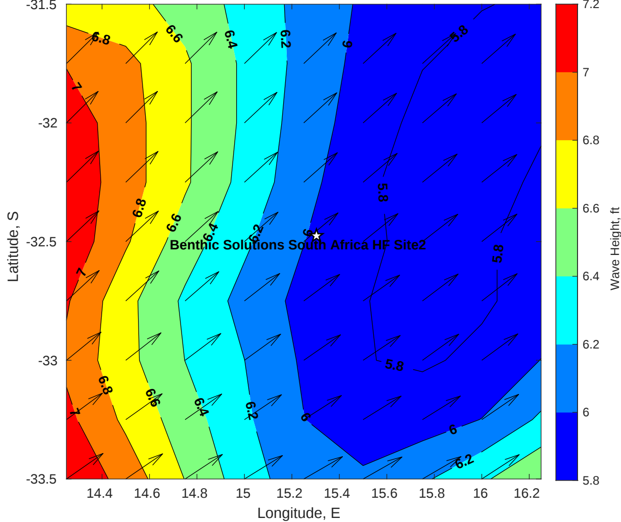
Wave Height (ft) for Benthic Solutions South Africa HF Site2 at 15-Jun-2025 09:00:00
