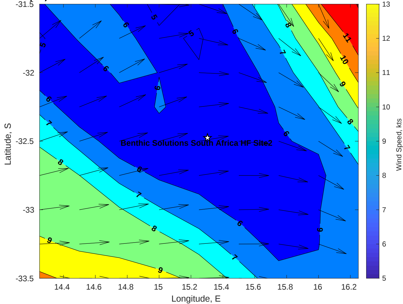
Winds (kts) for Benthic Solutions South Africa HF Site2 at 15-Jun-2025 09:00:00
