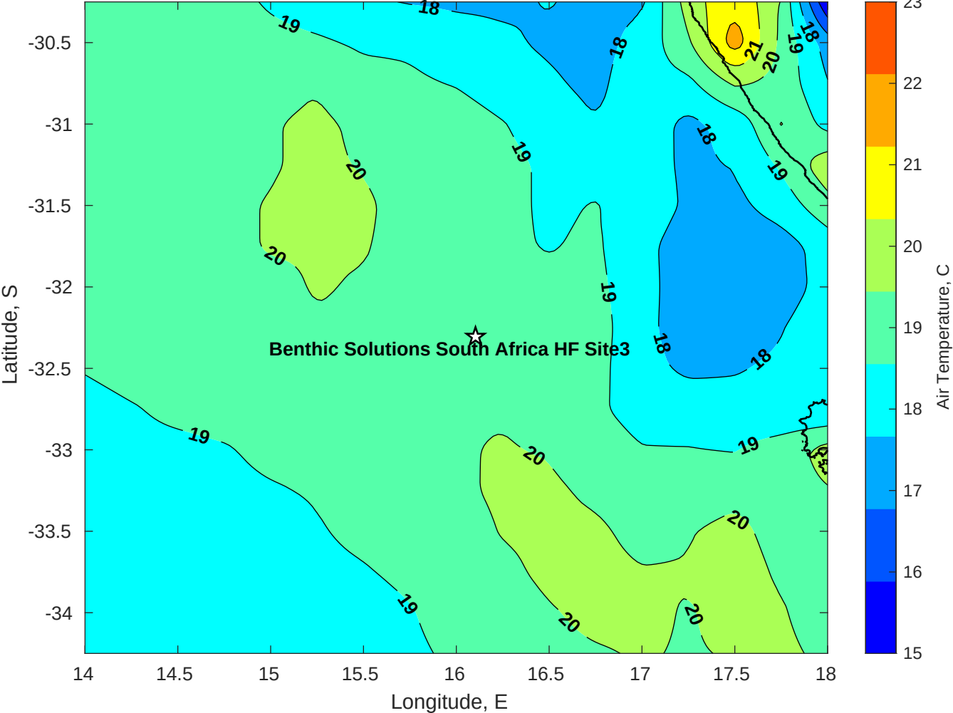
Air Temperature (C) for Benthic Solutions South Africa HF Site3 at 15-Jun-2025
