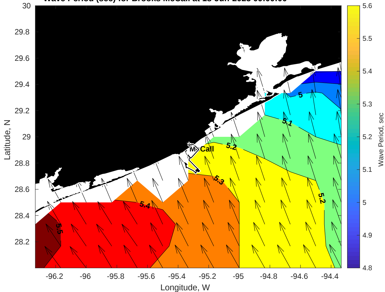
Wave Period (sec) for Brooks McCall at 18-Jun-2025 09:00:00
