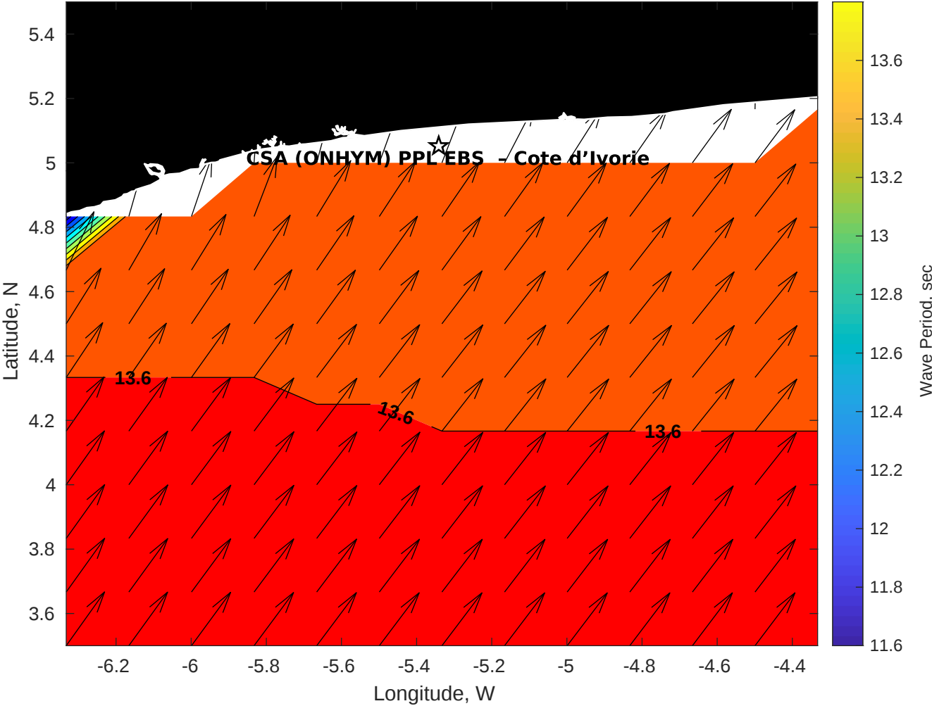
Wave Period (sec) for CSA (ONHYM) PPL EBS - Cote d'Ivoire at 15-Jun-2025 09:00:00
