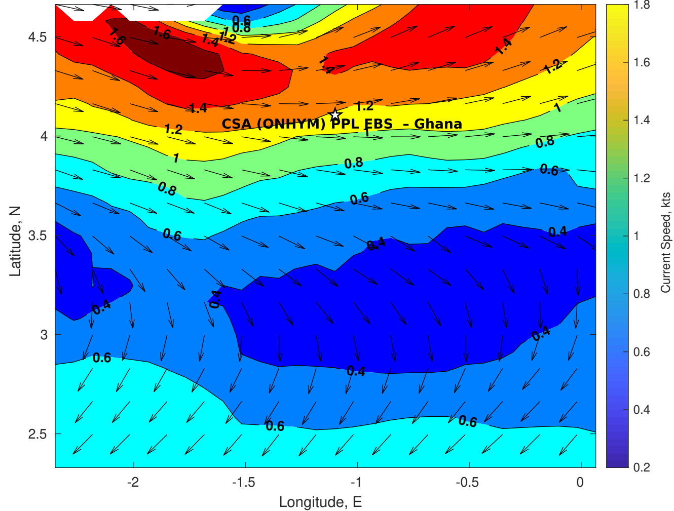
Surface Currents for CSA (ONHYM) PPL EBS - Ghana at 07-Jun-2025 00:00:00
