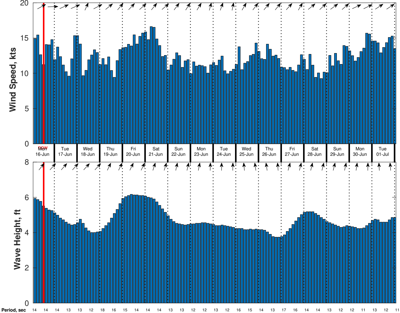
Wind & Wave Forecast for CSA (ONHYM) PPL EBS - Ghana from 15-Jun-2025 02:00:00 to 01-Jul-2025 02:00:00
