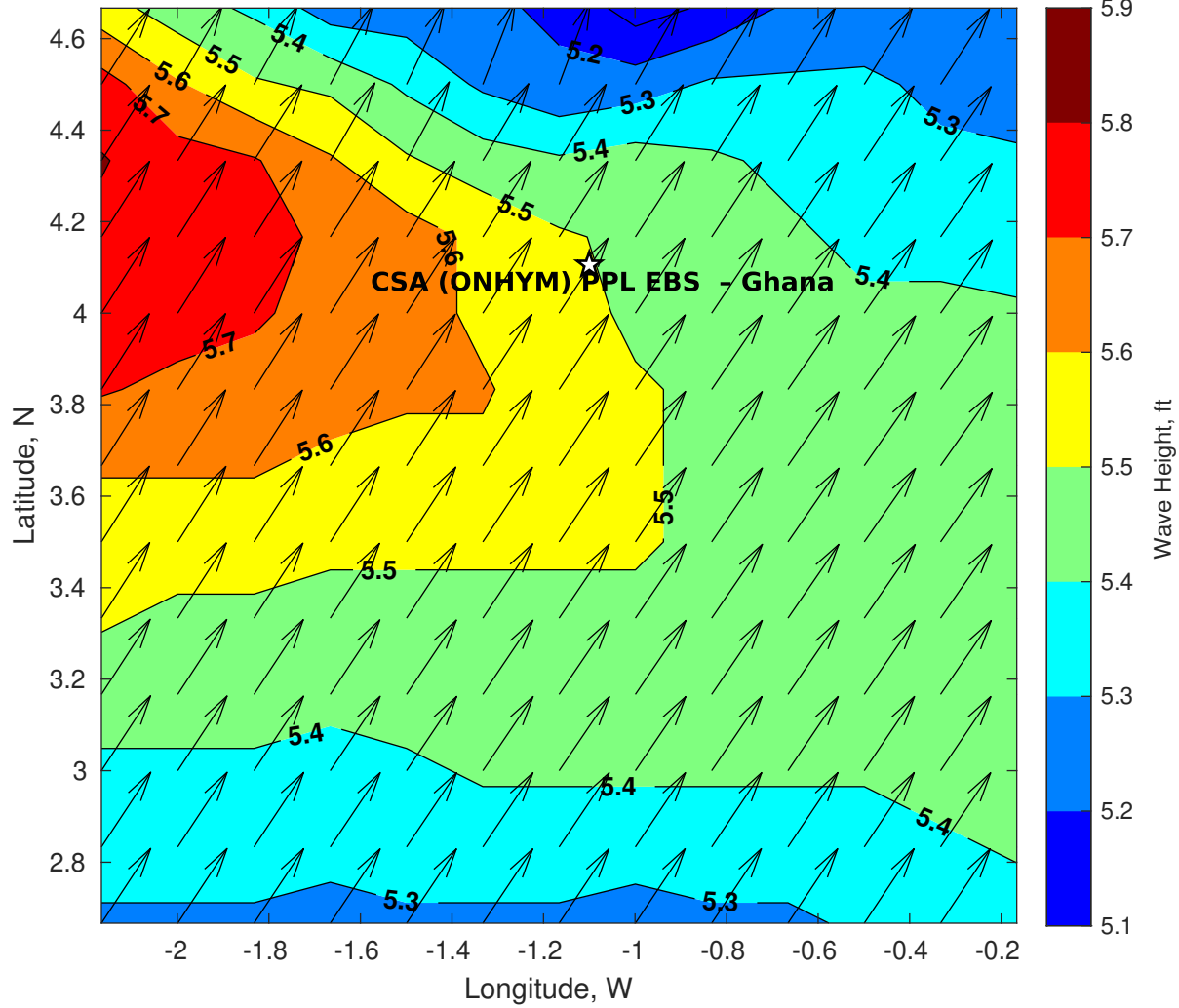
Wave Height (ft) for CSA (ONHYM) PPL EBS - Ghana at 15-Jun-2025 09:00:00
