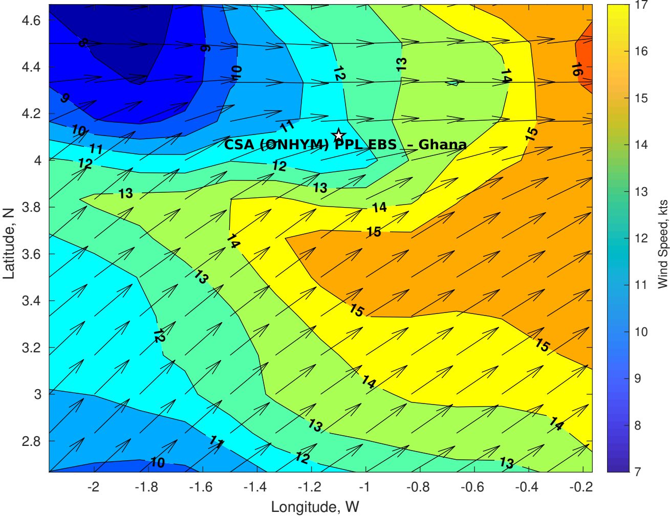
Winds (kts) for CSA (ONHYM) PPL EBS - Ghana at 15-Jun-2025 09:00:00
