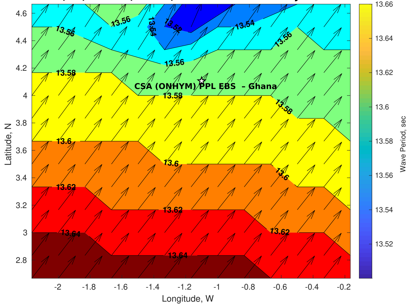
Wave Period (sec) for CSA (ONHYM) PPL EBS - Ghana at 15-Jun-2025 09:00:00
