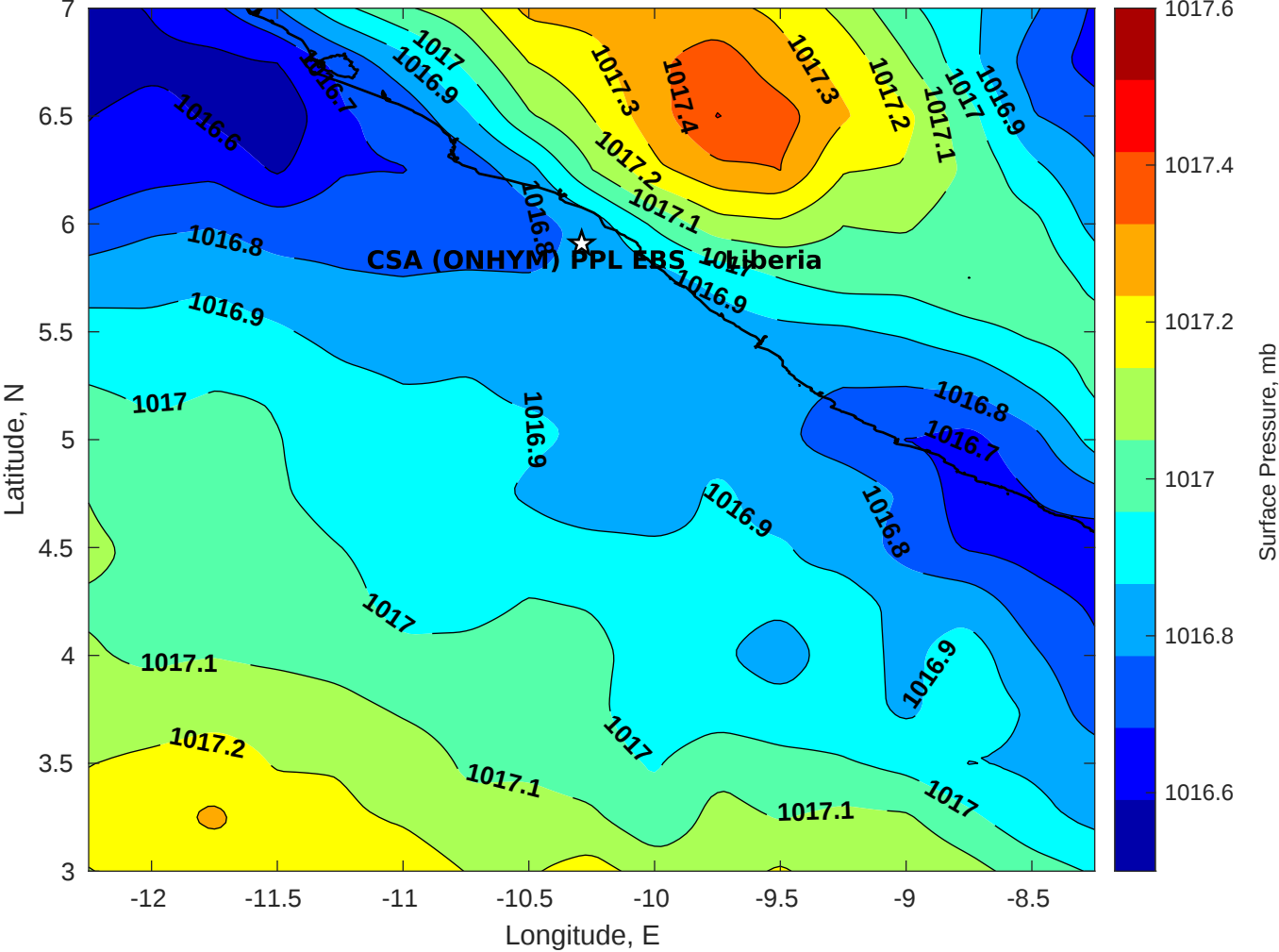
Surface Pressure (mb) for CSA (ONHYM) PPL EBS - Liberia at 17-Jun-2025 00:00:00
